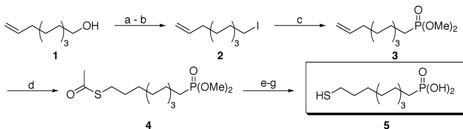
Scheme 1. (a) TsCl, Et 3 N, DMAP, CH 2 Cl 2 , 96%; (b) NaI, acetone, 96%; (c) P(OMe) 3 (10 equiv.), reflux, 95%; (d) thiolacetic acid, AIBN, Tol, reflux, 87%; (e) acetyl chloride, MeOH, 0°C, 85%; (f) TMS-Br; (g) H 2 O, 95% (two steps).
