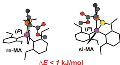
Figure 8. Transition states for si - and re -MA insertion into (\text{MeO})_2\mathbf{1} with a P helical configuration of the aromatic rings.
