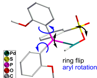
Figure 4. Observed molecular motions of (P^{\wedge}O)\text{Pd} complexes (fragment shown extracted from the X-ray structure of \text{MeO} \mathbf{1-OPBu}_3 ). 43
