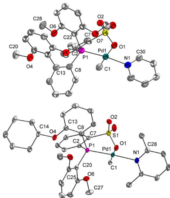
Figure 3. Solid-state structure of \text{Ar}/(\text{MeO})_2 \mathbf{1-py} (top) and of c\text{HexO}/(\text{MeO})_2 \mathbf{1-lut} . Ellipsoids represent 50% probability. Hydrogen atoms are omitted for clarity.
