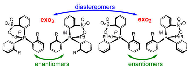
Figure 5. Helical chirality ( P , M ) as found for \text{Ar}_3\text{ZX} motifs and additional diastereomers for the case of ortho substitution of the aryl rings for [(\text{P}^{\text{Ar}}\text{O})\text{PdMe}] complexes.
