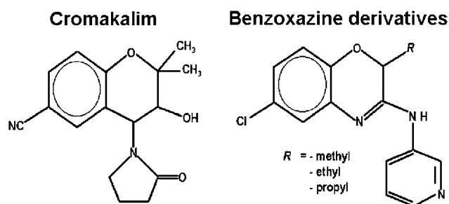
Figure 1 Chemical structures of cromakalim and of the newly synthesised benzoxazine derivatives. The 2H-1,4-benzoxazine derivatives are structural analogues of benzopyrans, the difference being the replacement of the carbon atom at position 4 with a nitrogen atom. The new molecules contain different alkyl substituents of variable length such as the methyl, ethyl and propyl at position 2 of the benzoxazine nucleus. All the synthesized molecules have a pyridylamino group with hydrogen bond forming capacity at position 3 and an electron-withdrawing group such as the chlorine atom at position 6 of the benzoxazine nucleus. The introduction of different alkyl substituents at position 2 of the benzoxazine ring gives the opportunity to evaluate the influence of the increase of lipophilicity and/or of alkyl chain length in this part of the molecule.
