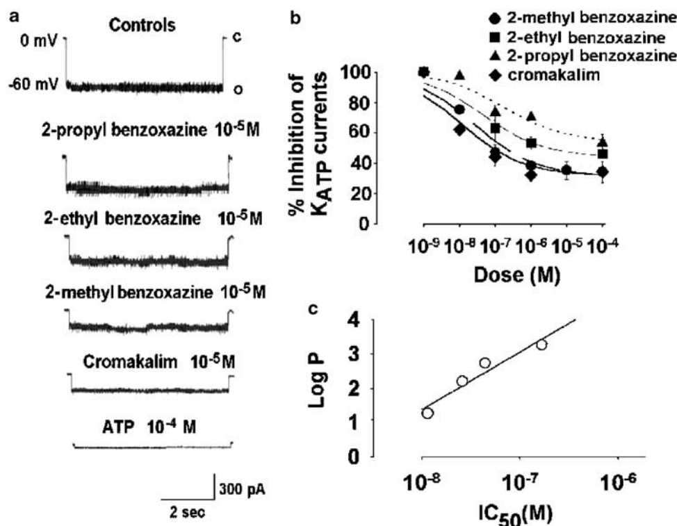
Figure 3 Effects of K^+ channel openers on K_{ATP} channels of rat skeletal muscle fibres in the absence of internal ATP. (a) Digital average of K_{ATP} current recorded in the excised inside-out macropatches, at -60 mV (V m), with high cytosolic KCl solutions on both sides of the membrane, in the absence (controls) ( n=26 macropatches), or in the presence of the 2 H -1,4-benzoxazine derivatives having the methyl ( n=5 macropatches), ethyl ( n=4 macropatches) or propyl ( n=6 macropatches) groups at position 2 on the benzoxazine ring or in the presence of cromakalim ( n=7 macropatches). C and O in the traces indicate closed and open channel levels, respectively. (b) Concentration-response relations of the 2 H -1,4-benzoxazine derivatives having the -CH_3 , -C_2H_5 or -C_3H_7 groups at position 2 of the benzoxazine ring, and of cromakalim on the K_{ATP} currents in the absence of ATP. All the compounds under investigation produced a concentration-dependent inhibition of the K_{ATP} current, (c) Log P plot versus the IC_{50} of the 2 H -1,4-benzoxazine derivatives and cromakalim. The calculated coefficient of correlation between the log P and IC_{50} of the compounds under investigation was 0.8.
