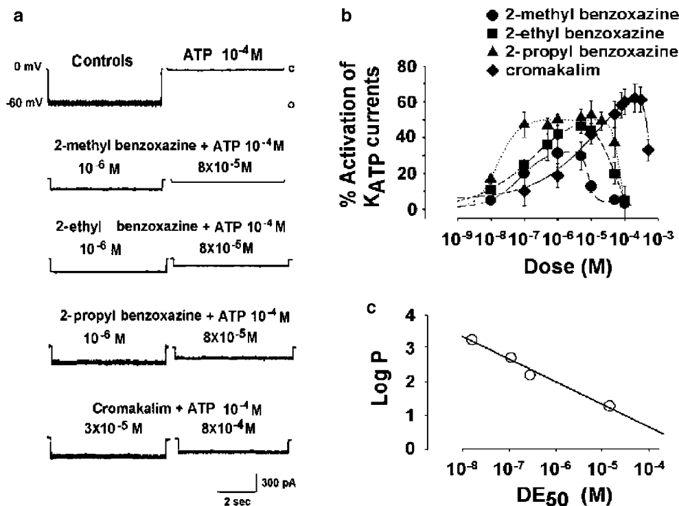
Figure 2 Effects of K^+ channel openers on K_{ATP} channels of rat skeletal muscle fibres in the presence of internal ATP. (a) Digital average of K_{ATP} current recorded in the excised inside-out macropatches, at -60 mV (V m), with high cytosolic KCl solutions on both sides of the membrane, in the absence (controls) ( n=31 macropatches), in the presence of 10^{-4} M concentration of ATP ( n=31 macropatches), in the presence of 10^{-4} M ATP + the 2H-1,4-benzoxazine derivatives having the methyl ( n=6 macropatches), ethyl ( n=5 macropatches) or propyl ( n=7 macropatches) groups at position 2 of the benzoxazine ring or in the presence of 10^{-4} M ATP + cromakalim ( n=4 macropatches). C and O in the traces indicate closed and open channel levels, respectively, (b) Concentration – response relation of the 2H-1,4-benzoxazine derivatives having the -CH 3 , -C 2 H 5 or -C 3 H 7 groups at position 2 of the benzoxazine ring, and of cromakalim on the K_{ATP} currents inhibited by a 10^{-4} M concentration of internal ATP. All the compounds under investigation including cromakalim produced a concentration-dependent increase of the K_{ATP} current at the lower doses, in contrast inhibiting it at the highest doses, (c) Log P plot versus the DE_{50} of the 2H-1,4-benzoxazine derivatives and cromakalim. An inverse relation was observed between the log P , as index of lipophilicity, and DE_{50} of the compounds under investigation showing a coefficient of correlation of -0.97 .
