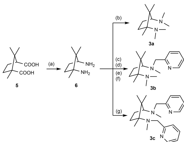
Scheme 2. (a) \text{NaCN} , \text{H}_2\text{SO}_4 , \text{CHCl}_3 , 55^\circ\text{C} , 77%. (b) Formic acid, formaldehyde, reflux, 83%. (c) Benzoyl chloride, EtOH 69%. (d) Formic acid, formaldehyde, reflux, 83%. (e) HCl reflux, 81%. (f) 1.) 2-Formylpyridine, \text{Na}_2\text{SO}_4 , MeOH, reflux 2.) \text{NaBH}_4 , MeOH 3.) Formaldehyde, \text{NaCNBH}_3 , MeOH 72%. (g) 1.) 2-Formylpyridine, \text{Na}_2\text{SO}_4 , MeOH, reflux 2.) \text{NaBH}_4 , MeOH 3.) Formaldehyde, \text{NaCNBH}_3 , MeOH 26%.
