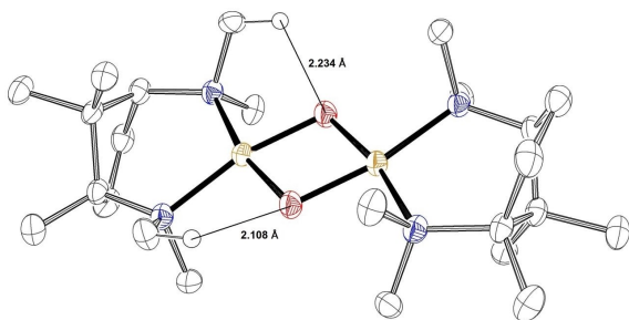
Figure 7. Molecular structure of [\text{Cu}_2(3\text{ad}_{12})_2\text{O}_2]^{2+} . Hydrogen atoms (except the nearest C–H's to O), the \text{PF}_6 anions and solvent molecules are omitted for clarity. Ellipsoids are drawn at 50% probability.
