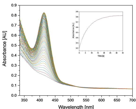
Figure 6. Time-resolved UV/Vis spectra of the reaction of [\text{Cu}(\text{3a})]\text{OTf} ( c = 0.5 \times 10^{-3} \text{ M} ) with dioxygen ( c = 2.15 \times 10^{-3} \text{ M} ) in DCM at -89^\circ\text{C} for 35 s. The inset shows the absorbance vs time at \lambda = 414 \text{ nm} .
