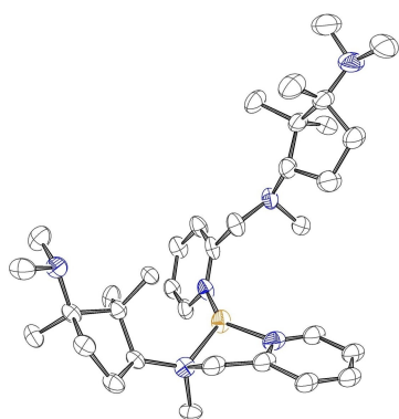
Figure 3. Molecular Structure of [\text{Cu}(\mathbf{3b})]^+ . Hydrogen atoms and perchlorate anion are omitted for clarity. Ellipsoids are drawn at 50% probability.
