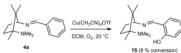
Scheme 7. First attempt at hydroxylation of ligand 4a . Conversion was determined using the integral of the imine proton signals.
