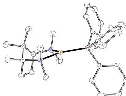
Figure 2. Molecular Structure of [\text{Cu}(\text{3a})(\text{PPh}_3)]^+ . Hydrogen atoms and the triflate anion are omitted for clarity. Ellipsoids are drawn at 50% probability.
