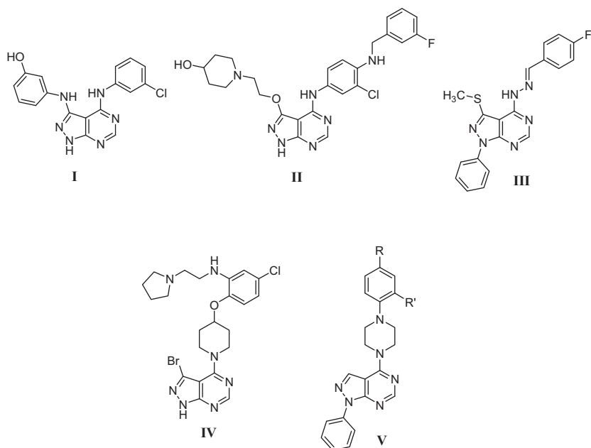
Chart 1: Examples of some pyrazolo[3,4- d ] pyrimidines with antitumor activity.
