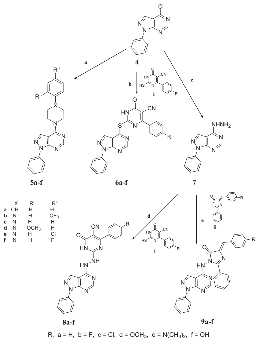
Scheme 2: Synthesis of compounds 5a-f , 6a-f , 7 , 8a-f , and 9a-f . Reagents and reaction conditions. (a) Phenylpiperidine/ appropriate phenylpiperazine, dry DMF, triethylamine, reflux 15 h; (b) appropriate derivative i , absolute ethanol, anh. K 2 CO 3 , reflux 20 h; (c) NH 2 NH 2 ·H 2 O, ethanol, reflux, 2.5 h; (d) appropriate derivative i , dry DMF, TEA, reflux, 20 h; (e) appropriate derivative ii , gl. acetic acid, fused CH 3 COONa, boiling water bath, 3 h.
