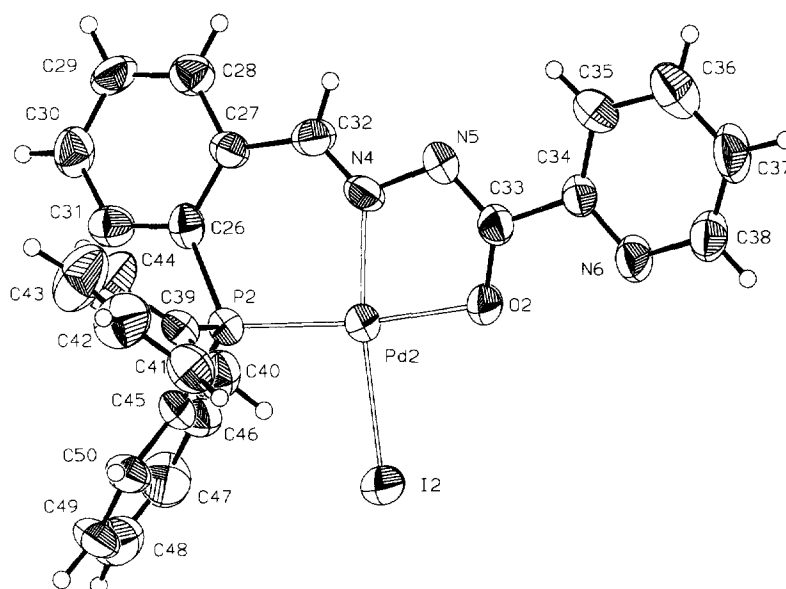
Fig. 4. ORTEP diagram for \text{Pd}(\text{pidf})\text{I} (molecule B). Thermal ellipsoids are drawn at the 50% probability level. Hydrogen atoms are represented by arbitrarily small spheres.
