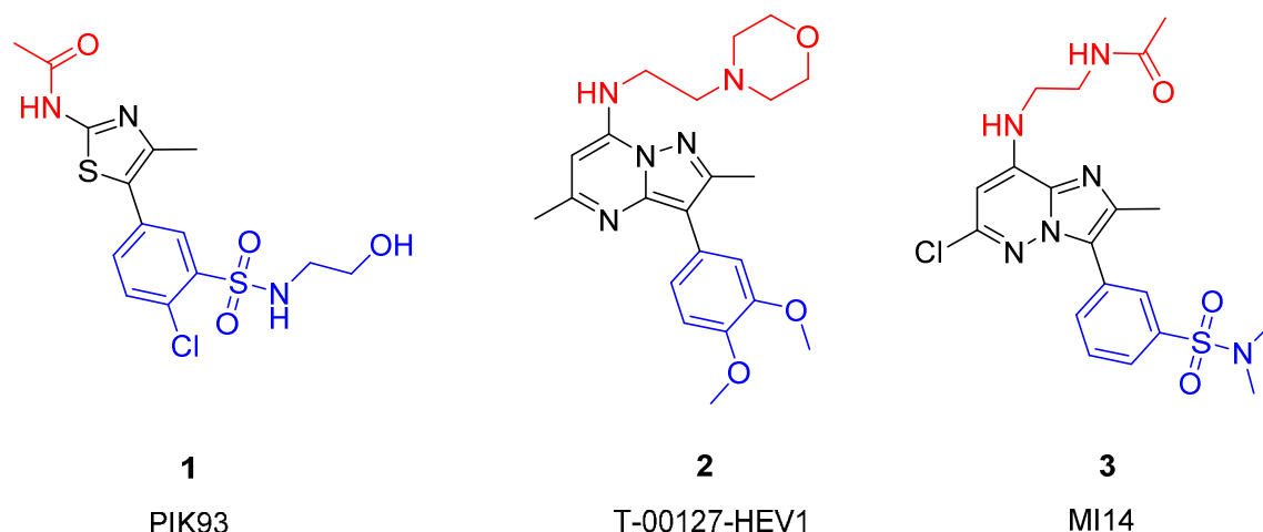
Figure 1. Structures of PI4KB inhibitors.
