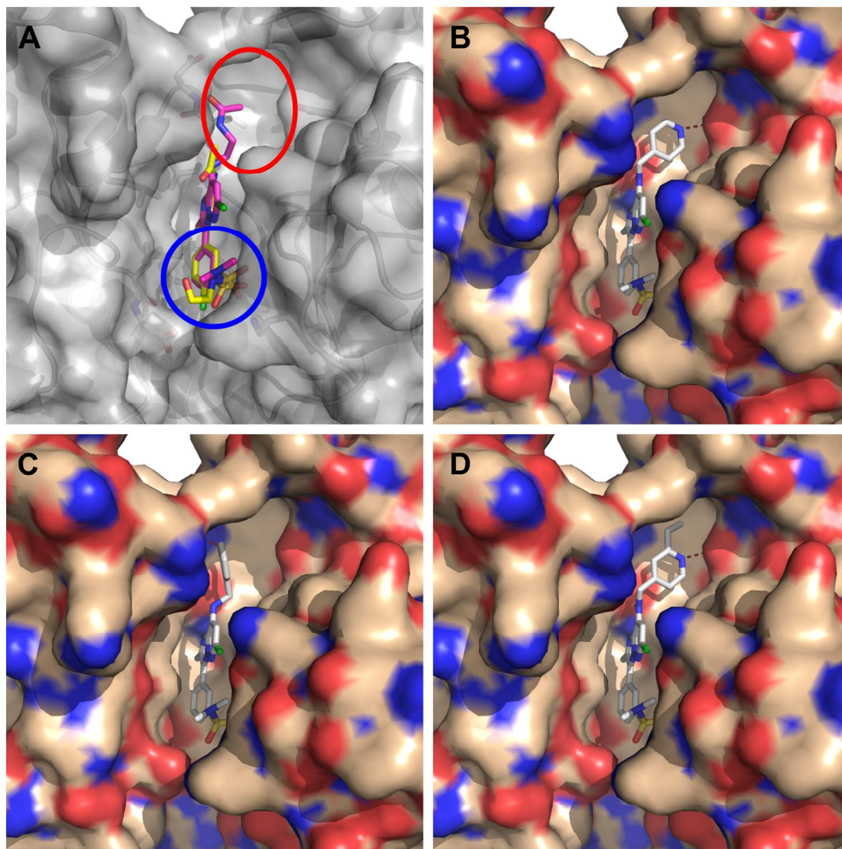
Figure 2. Design of new series of PI4KB inhibitors. A) Overlay of the crystal structure of PI4KB with 1 (yellow) and the docking model of the preferred conformation of 3 (magenta) unveils two sites of possible modifications. The red region can easily accommodate a large aromatic substituent. The blue region appears open for further optimization of the aromatic part of the molecule. B-D) Docking poses of derivatives 4 , 5 , and 8 , respectively. The figure was prepared using PyMOL.
