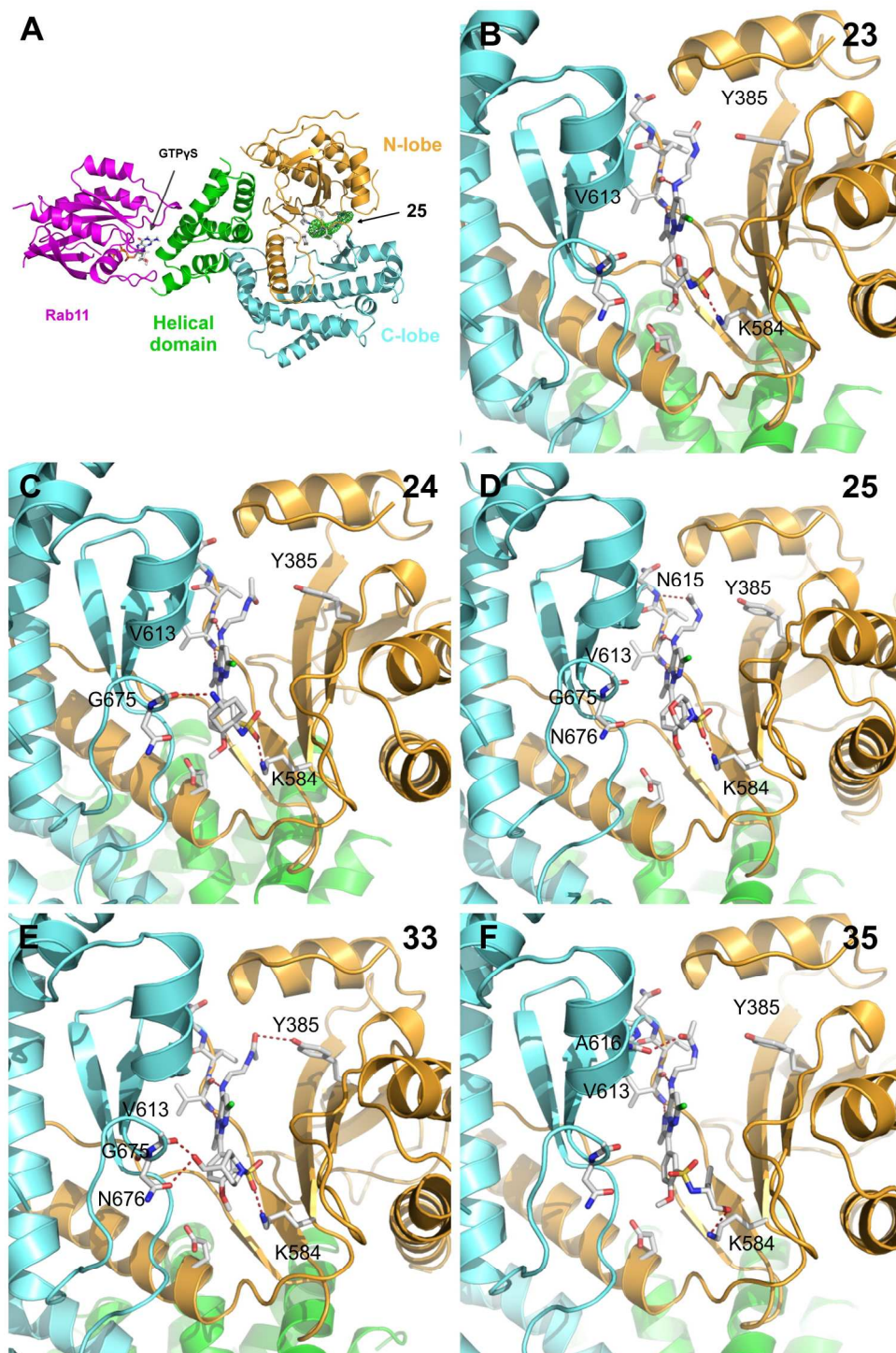
Figure 4. Structural analysis of newly the prepared inhibitors. A) Structure of the whole crystalized complex of PI4KB with Rab11. B-F) Binding modes of inhibitors 23 , 24 , 25 , 33 , and 35 . The figure was prepared using PyMOL.
