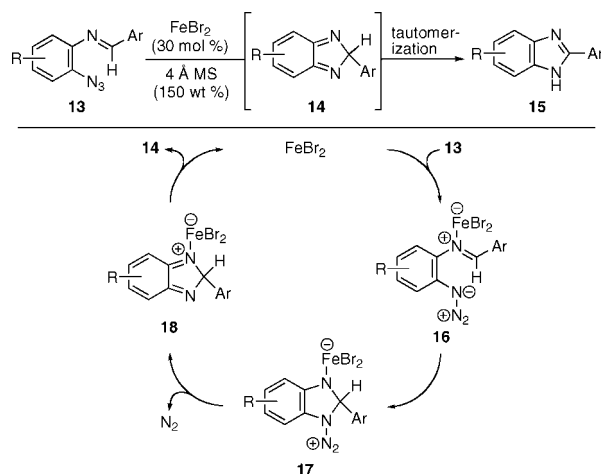
Scheme 4. Potential Mechanism for Benzimidazole Formation
