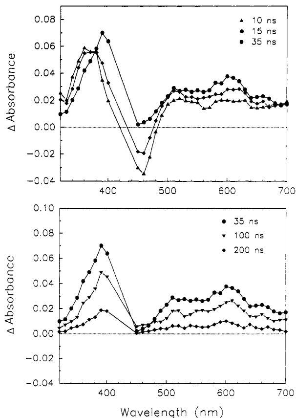
Figure 6. Nanosecond transient absorption difference spectra obtained following 420-nm, 4-ns pulsed ( \leq 5.2 \text{ mJ/pulse} ) excitation of a CH 3 CN solution \sim 1 \times 10^{-5} \text{ M} in 1, [PTZpn-Lys(Ru II b 2 m) 2+ -NH-prPQ 2+ ] at 25 °C. Top panel: rise of transient spectrum; bottom panel: decay of transient spectrum.
