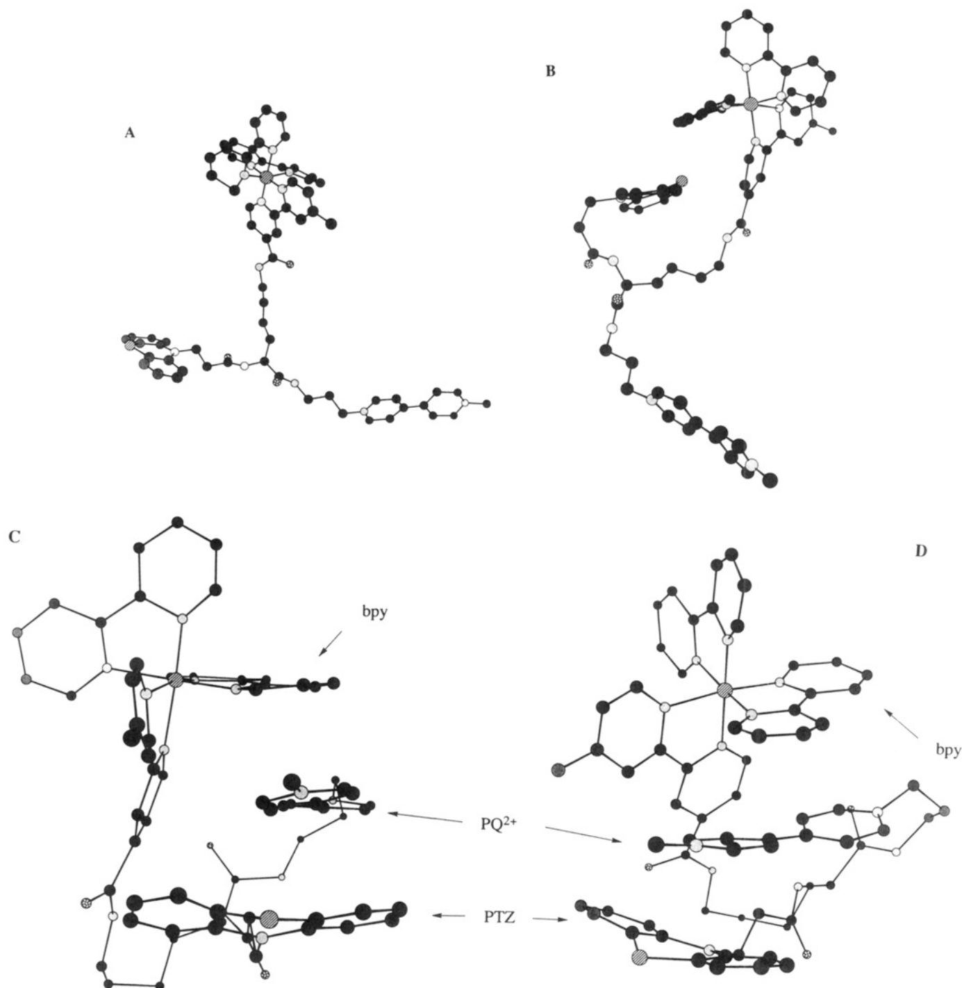
Figure 10. Selected conformations of triad 1 obtained from the dynamics calculation: 48 (A) an extended conformation; (B) a partially folded conformation in which PTZ is stacked beneath one of the bpy ligands of the chromophore; (C) a folded conformation in which PQ 2+ is stacked between PTZ and bpy; and (D) a rotated view of the same structure shown in (C). The hydrogen atoms are not displayed. Note that either PQ 2+ or PTZ can fold into the central position.
