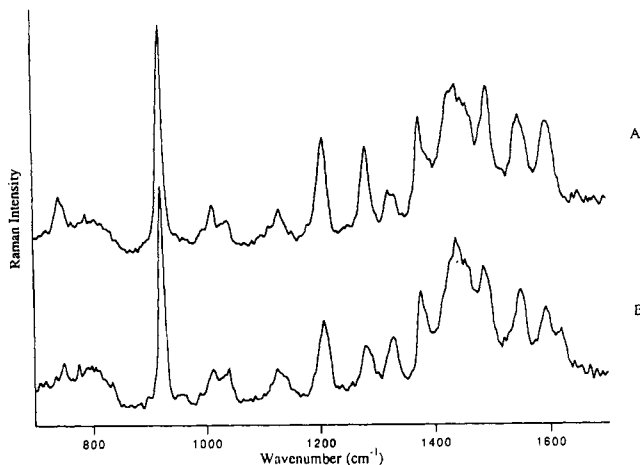
Figure 3. Time-resolved resonance Raman spectra of 3 , [\text{Ru}^{\text{II}}\text{b}_2\text{m-NHCH}_3]^{2+} (A, upper spectrum) and [\text{Ru}^{\text{II}}(\text{m-NHCH}_3)_3]^{2+} (B, lower spectrum) in \text{CH}_3\text{CN} . The spectra were measured as described in the Experimental Section and represent a total integration time of 16 min. Excited-state Raman peaks for \text{m-NHCH}_3 appear at 745, 1012, 1037, 1131, 1209, 1283, 1429, 1441, 1494, and 1552\text{ cm}^{-1} . Peaks at 1327 and 1598\text{ cm}^{-1} are ground-state bpy (b) peaks. Solvent peaks appear at 923 and 1377\text{ cm}^{-1} .
