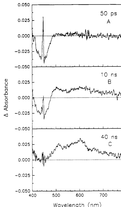
Figure 4. Picosecond transient absorption spectra recorded after excitation of a 5 \times 10^{-5} \text{ M} solution of 1, [PTZpn-Lys(Ru II b 2 m) 2+ -NH-prPQ 2+ ], in CH 3 CN with a 447-nm, 25-ps laser pulse. A mask was used at the face of the SIT detector to minimize the amount of 447-nm excitation reaching the detector and is responsible for the “notch” in the picosecond data in the 447-nm region. Each difference absorption spectrum is the average of the result of \sim 400 excitation laser shots. The average excitation pulse energy was 0.186 mJ/pulse. The energy dependence of the signal intensity was linear in this energy regime.
