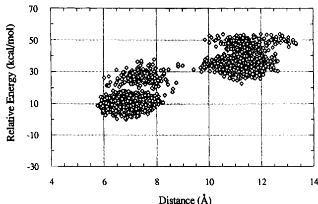
Figure 9. Distribution plot of relative energy vs distance (Å) of edge-to-edge separation between \text{PTZ} and \text{PQ}^{2+} in triad 1 . Note that the folded conformations (separation distance of 6–8 Å) have somewhat lower energy than more extended conformations (distances of 10.5–12.5 Å).
