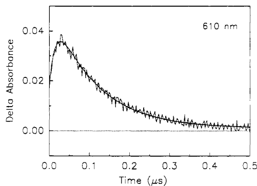
Figure 7. Fitted decay trace for data obtained at 610 nm. The smooth curve is the computer-generated fit to a biexponential function with rate constants of k = (6.82 \pm 0.07) \times 10^7 \text{ s}^{-1} ( \tau = 14.7 \pm 1 \text{ ns} ) and (9.26 \pm 0.03) \times 10^6 \text{ s}^{-1} ( \tau = 108 \pm 1 \text{ ns} ).
