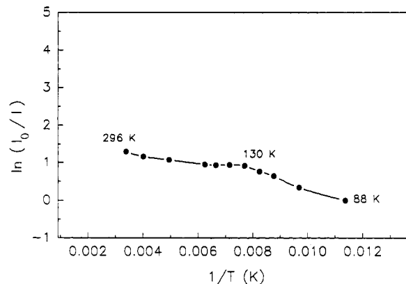
Figure 2. Temperature-dependent emission data for 3 , [Ru II b 2 m-NHCH 3 ] 2+ , in 4:1 ethanol/methanol. Each data point represents the integrated emission intensity over the range of 500–800 nm at a selected temperature, and the data set is normalized to the integrated emission intensity at 88 K.
