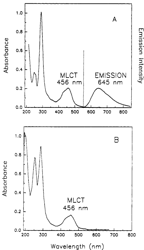
Figure 1. (a) UV-visible absorption spectra (normalized, left axis) and emission spectra (scaled arbitrarily, right axis) in CH 3 CN for 3 , [Ru II b 2 m-NHCH 3 ] 2+ . (b) Normalized UV-visible absorption spectra in CH 3 CN for 1 , [PTZpn-Lys(Ru II b 2 m) 2+ -NH-prPQ 2+ ]. Samples were \sim 5 \times 10^{-4} M with \epsilon_{456 \text{ nm}} = 11\,700 L mol -1 cm -1 and were the PF 6 - salts.
