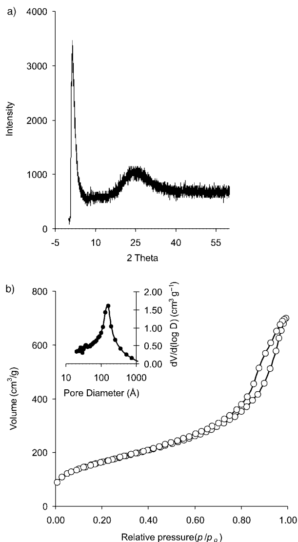
Figure 1. a) Powder XRD ( \text{Cu}_{\text{K}\alpha} ) pattern of AITUD-1; b) nitrogen sorption isotherms of AITUD-1. Inset: corresponding pore-size distribution.
