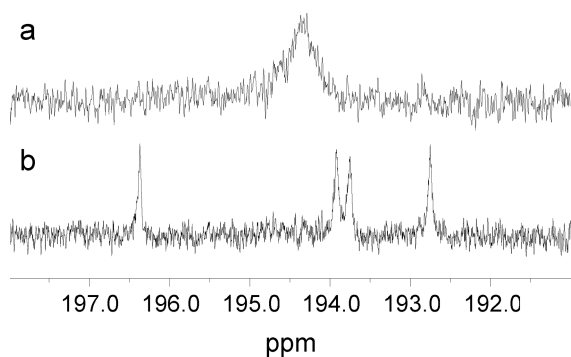
Figure 4. ^{13}\text{C} NMR spectra of (\text{acrylic acid})\text{Ru}(\text{CO})_4 in \text{CDCl}_3 at (a) 20^\circ\text{C} (194.3 ppm) and (b) -40^\circ\text{C} (192.7, 193.7, 193.9, and 196.4 ppm).
