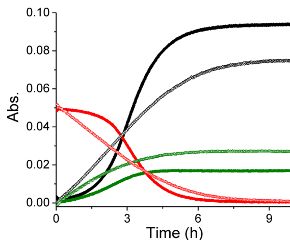
Figure 12. Reaction profiles for (\text{CH}_2=\text{CHCOOH})\text{Fe}(\text{CO})_4 + 10 equiv of \text{PPh}_3 in chlorobenzene at 333 K, (acrylic acid) \text{Fe}(\text{CO})_4 (red), (\text{PPh}_3)\text{Fe}(\text{CO})_4 (green), and \text{trans}-(\text{PPh}_3)_2\text{Fe}(\text{CO})_3 (black). Solid line in absence of piperidine, and hollow line in presence of 1 equiv of piperidine.
