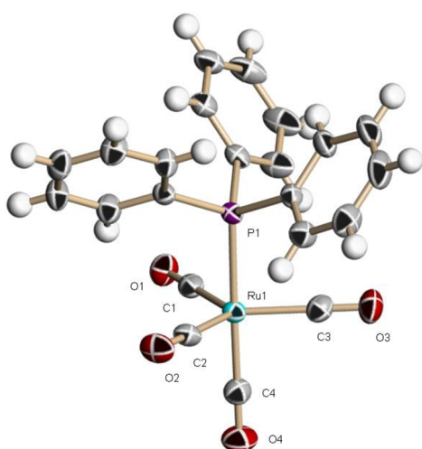
Figure 6. Thermal ellipsoid representation of the X-ray structure of (PPh 3 )Ru(CO) 4 with ellipsoids at 50% probability surfaces.
