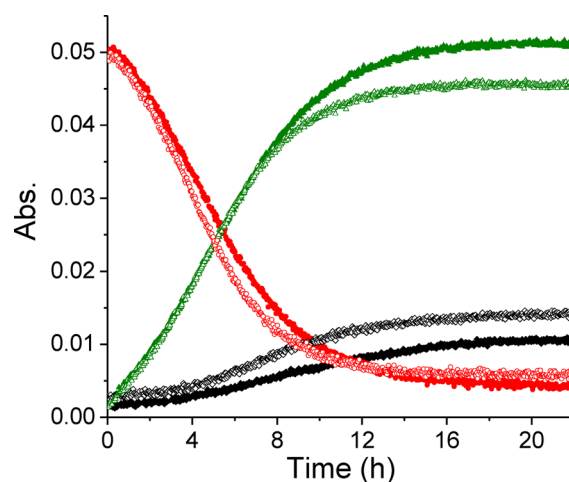
Figure 7. Infrared \nu_{\text{CO}} profiles for (acrylic acid)Ru(CO) 4 disappearance (red) and appearance of (PPh 3 )Ru(CO) 4 (green) and trans -(PPh 3 ) 2 Ru(CO) 3 (black). Ten-fold excess PPh 3 (solid lines) and 30-fold [PPh 3 ] (hollow lines) in CH 2 Cl 2 at 283 K.
