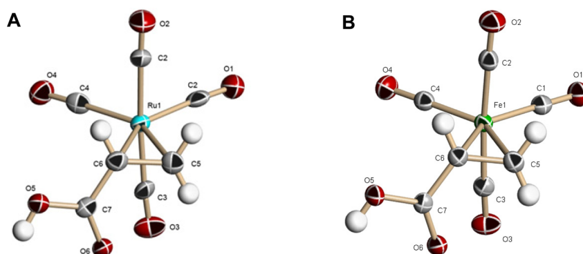
Figure 1. X-ray structures: Thermal ellipsoid representations of A , (\text{CH}_2=\text{CHCOOH})\text{Ru}(\text{CO})_4 , and B , (\text{CH}_2=\text{CHCOOH})\text{Fe}(\text{CO})_4 with ellipsoids at 50% probability surfaces.
