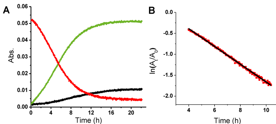
Figure 5. (A) Infrared \nu_{\text{CO}} peak profiles as a function of time for (acrylic acid)Ru(CO) 4 (red), (PPh 3 )Ru(CO) 4 (green), and trans -(PPh 3 ) 2 Ru(CO) 3 (black) at 283 K in CH 2 Cl 2 . (B) Plot of \ln(A_t/A_0) vs time for disappearance of (acrylic acid)Ru(CO) 4 , R^2 = 0.997 .
