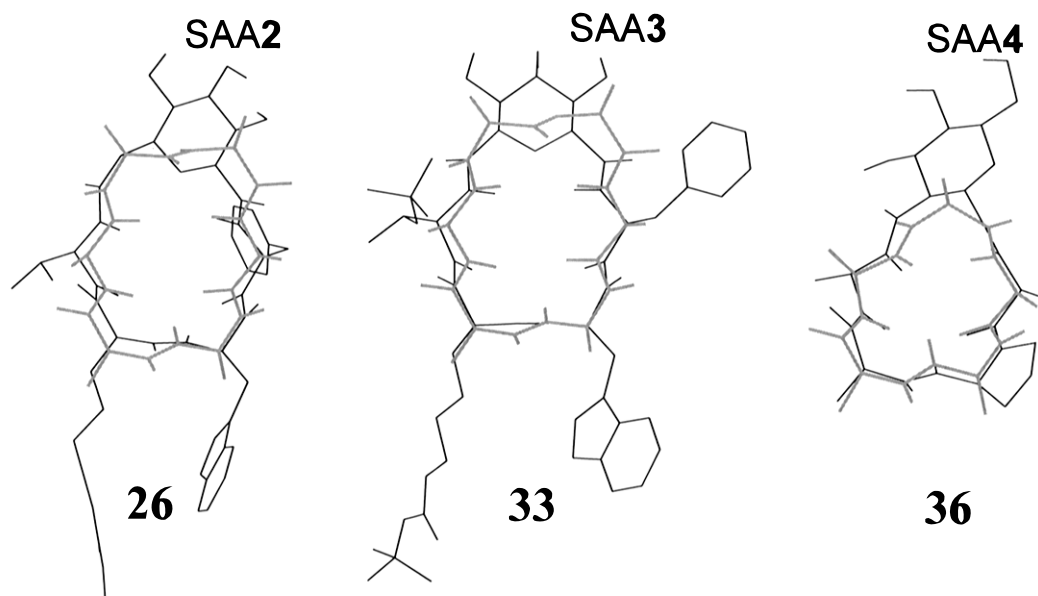
Figure 9. Superposition of 26 (black) and an idealized \beta\text{II}'/\beta\text{II}' -turn arrangement (gray); superposition of 33 (black) and an idealized \beta\text{II}'/\beta\text{II}' -turn arrangement (gray); and superposition of 36 (black) and an idealized \beta\text{II}'/\gamma -turn-arrangement (gray).
