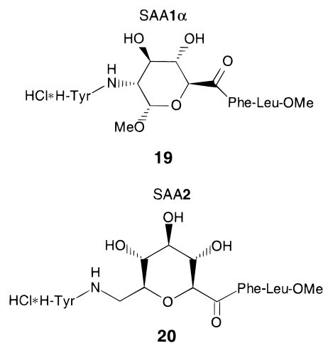
Figure 3. SAA1 \alpha and SAA2 incorporated into enkephalin analogs 19 and 20 .
