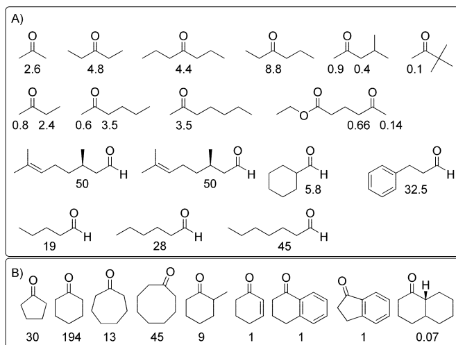
Figure 2. Ketone and aldehyde substrates used for 38C2-catalyzed deuterium exchange reactions at the \alpha -carbon. The numbers, taken from reference [12], are rate constants ( \text{min}^{-1} ). When two numbers are given for one substrate, they refer to the \alpha - and \alpha' -positions. A) Acyclic ketones and aldehydes. B) Cyclic ketones.
