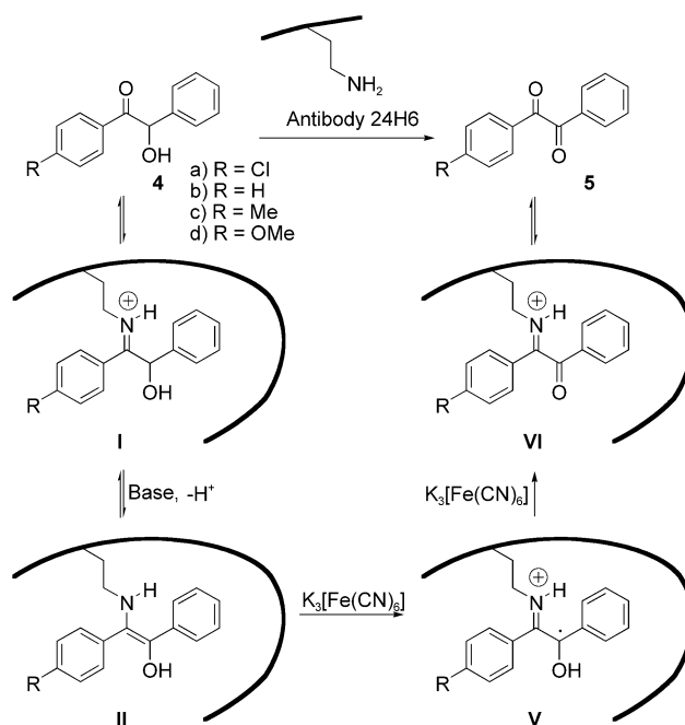
Scheme 4. Mechanistic pathway of the antibody-catalyzed oxidation reaction.
