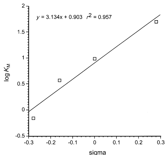
Figure 5. \log(K_M) versus \sigma for the oxidation reaction.
