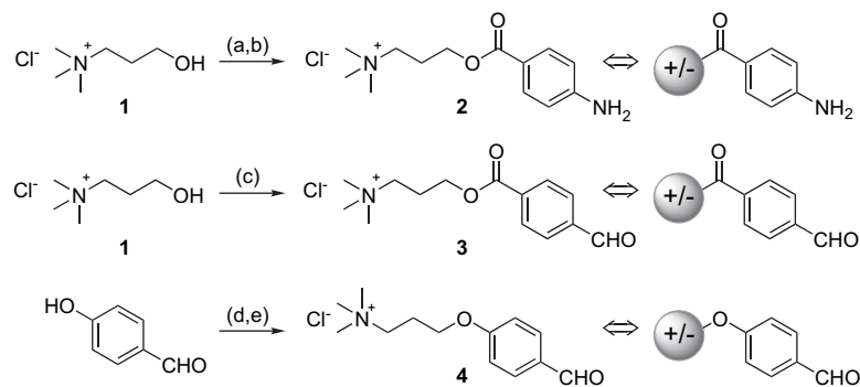
Scheme 1. Preparation of ammonium chloride supported aniline and benzaldehyde. (a) 4-NO 2 C 4 H 6 CO 2 H, DCC, DMAP, CH 3 CN, rt; (b) Pd/C, H 2 (5 bar), H 2 O, rt, 92% (over two steps); (c) 4-CHOC 4 H 6 CO 2 H, DCC, DMAP, CH 3 CN, rt (96%); (d) Br(CH 2 ) 3 Cl, K 2 CO 3 , acetone, Δ, 87%; (e) NMe 3 (50% aqueous), CH 3 CN, 70 °C, 18 h, 98%.
