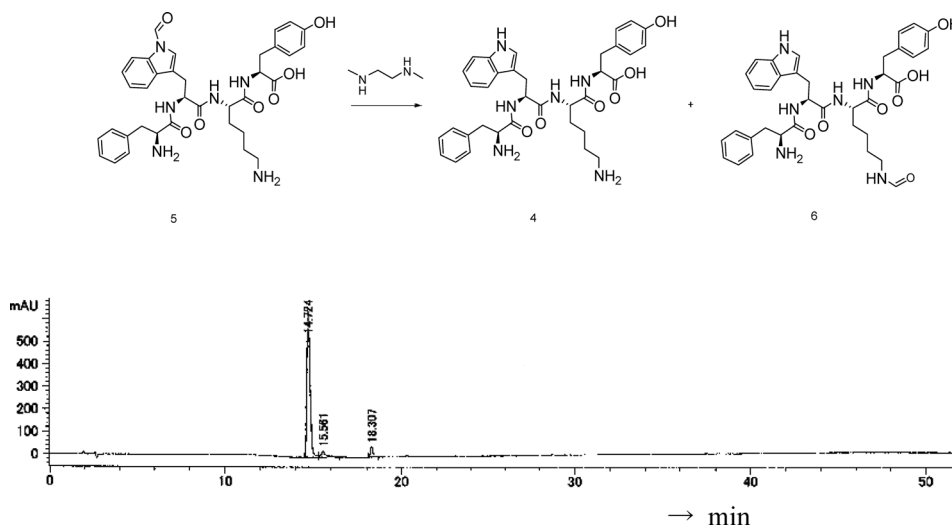
Fig. 3. Summary of the Deprotection of the Model Peptide with N,N' -Dimethylethylenediamine (DMEDA) in Water and HPLC Profile for Compounds 4 — 6
