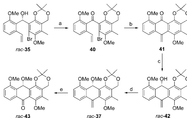
Scheme 6. Synthesis of tricycle rac - 43 . a) Dess–Martin periodinane, CH 2 Cl 2 , 20^{\circ}\text{C} , 15 min, 81%; b) n Bu 4 NOAc, DMF/CH 3 CN/H 2 O, 60^{\circ}\text{C} , then Herrmann–Beller catalyst, 110^{\circ}\text{C} , 17 h, 74%; c) LiAlH 4 , THF, 0^{\circ}\text{C} , 10 min; d) NaH, MeI, THF, 0^{\circ}\text{C} → 20^{\circ}\text{C} , 14 h, 37% over two steps; e) RuCl 3 , NaIO 4 , CCl 4 , MeCN, H 2 O, 0^{\circ}\text{C} , 15 min, 69%.
