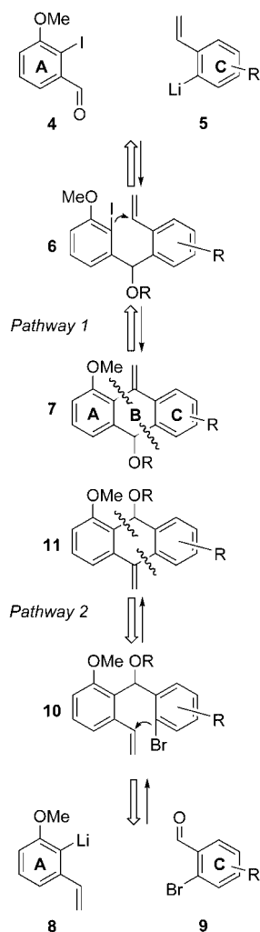
Scheme 1. Retrosynthesis analysis of the carbocyclic core of mensacarcin ( 1 ).
