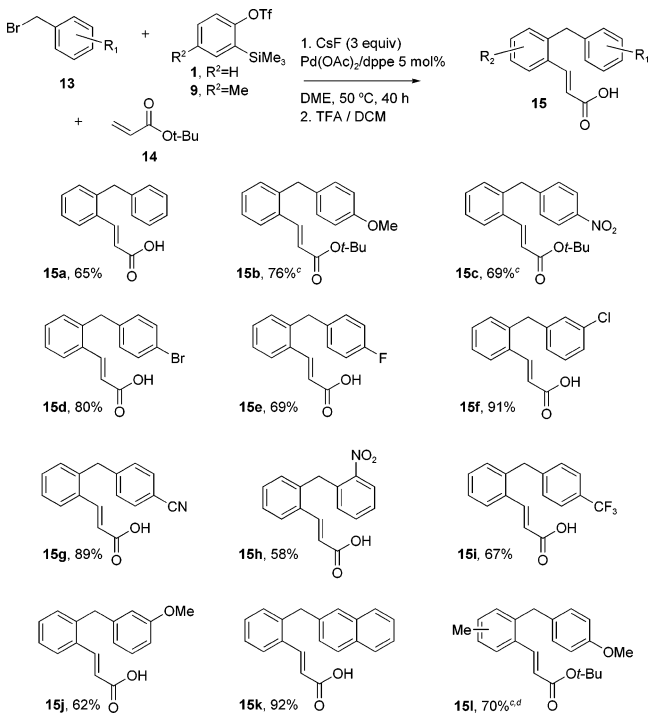
Chart 2. Three-Component Coupling of Benzyl Bromides, Benzyne, and tert -Butyl Acrylate a,b
