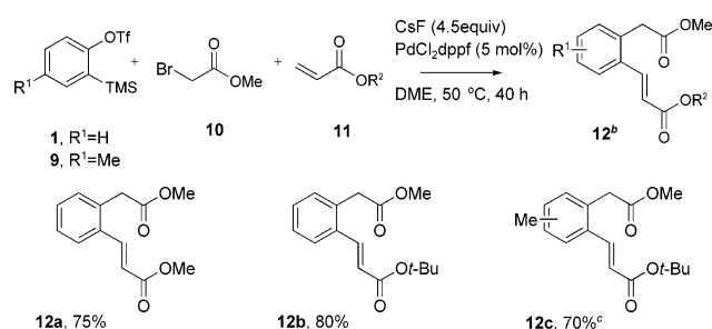
Chart 1. Three-Component Coupling of Benzyne, Methyl Bromoacetate, and an Acrylate a
