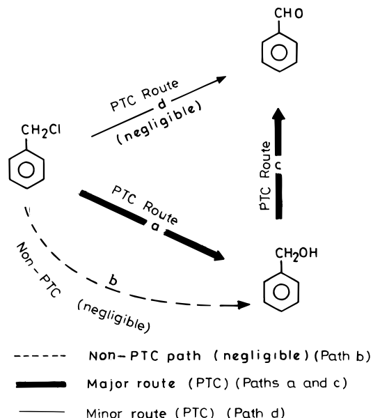
Figure 3. Triangular paths of reaction. The PT catalysis path is due to the formation of [\text{Q}^+\text{HCrO}_4^-]_{\text{org}} .
