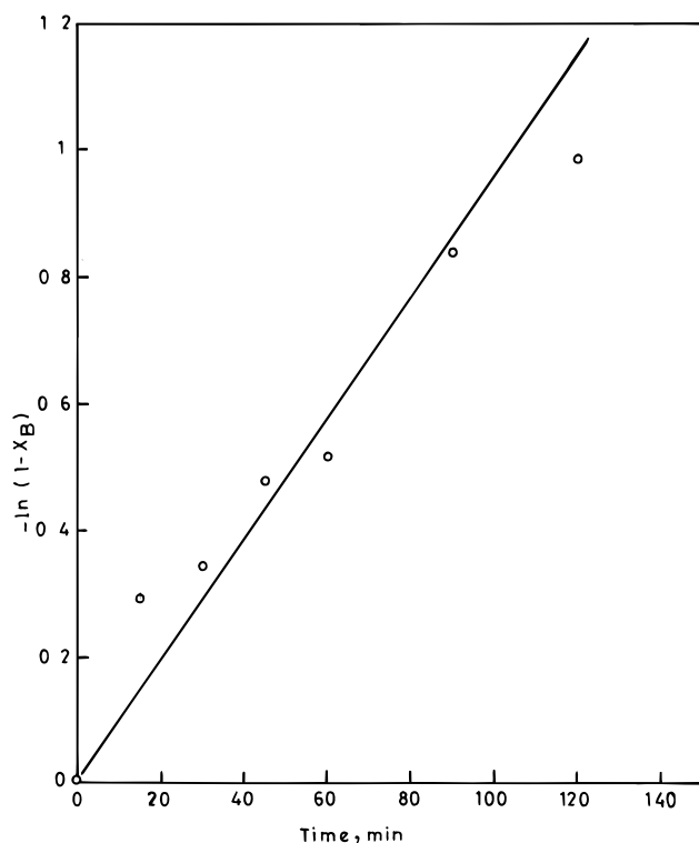
Figure 6. Kinetics of plot of oxidation of benzyl alcohol with \text{HCrO}_4^- under PTC catalysis conditions. Speed = 1000 rpm. Temperature = 100 °C. [\text{BnOH}] = 1.09 \times 10^{-3} \text{ mol/cm}^3 , [\text{K}_2\text{Cr}_2\text{O}_7] = 9.33 \times 10^{-4} \text{ mol/cm}^3 , \text{Vol}_{\text{org}} = \text{Vol}_{\text{aq}} = 50 \text{ mL} , [\text{Na}_2\text{CO}_3] = 4.44 \times 10^{-4} \text{ mol/cm}^3 , [\text{TBAB}]_{\text{org}} = 9.32 \times 10^{-5} \text{ mol/cm}^3 .
