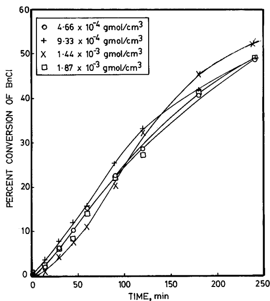
Figure 13. Effect of concentration of nucleophile HCrO_4^- on rate of reaction of benzyl chloride. Speed = 1000 rpm. Temperature = 100 °C. [BnCl] = 1.86 \times 10^{-3} mol/cm 3 . Vol_{org} = Vol_{aq} = 50 mL. [Na_2CO_3] = 4.44 \times 10^{-4} mol/cm 3 . [TBAB]_{org} = 9.32 \times 10^{-5} mol/cm 3 .
