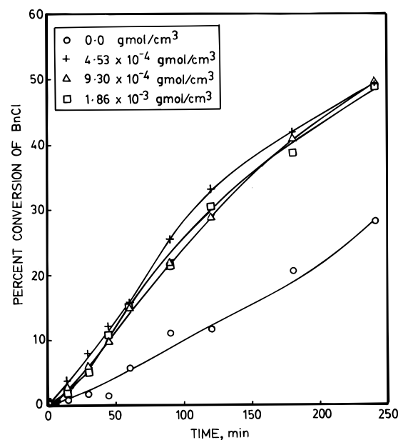
Figure 15. Effect of addition of sodium carbonate on conversion of benzyl chloride. Speed = 1000 rpm. Temperature = 100 °C. [BnCl] = 1.86 \times 10^{-3} mol/cm 3 . [K_2Cr_2O_7] = 9.33 \times 10^{-4} mol/cm 3 . Vol_{org} = Vol_{aq} = 50 mL. [TBAB]_{org} = 9.32 \times 10^{-5} mol/cm 3 .
