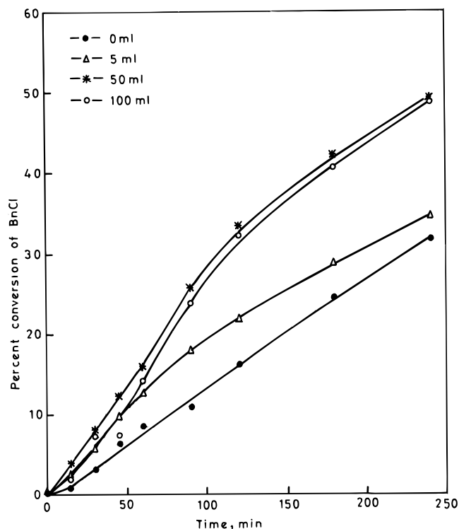
Figure 16. Effect of amount of water on conversion of benzyl chloride. Speed = 1000 rpm. Temperature = 100 °C. [BnCl] = 1.86 \times 10^{-3} mol/cm 3 . [K_2Cr_2O_7] = 9.33 \times 10^{-4} mol/cm 3 . Vol_{org} = 50 mL. [Na_2CO_3] = 4.44 \times 10^{-4} mol/cm 3 . [TBAB]_{org} = 9.32 \times 10^{-5} mol/cm 3 .
