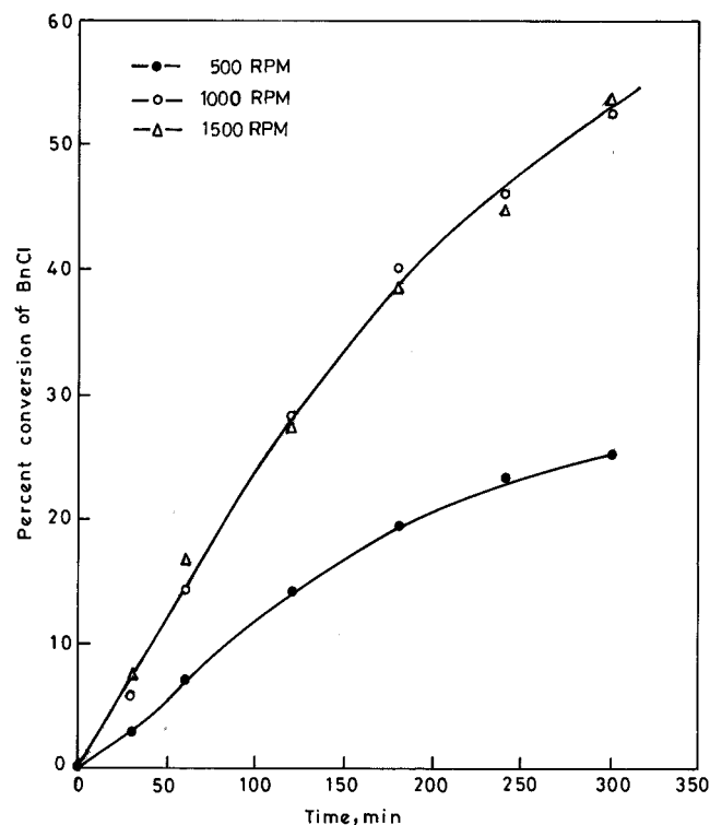
Figure 2. Effect of speed of agitation on conversion of benzyl chloride. Temperature = 100 °C. [\text{BnCl}] = 1.86 \times 10^{-3} \text{ mol/cm}^3 of organic phase. [\text{K}_2\text{Cr}_2\text{O}_7] = 9.33 \times 10^{-4} \text{ mol/cm}^3 of aqueous phase. \text{Vol}_{\text{org}} = \text{Vol}_{\text{aq}} = 50 \text{ mL} . [\text{Na}_2\text{CO}_3] = 4.44 \times 10^{-4} \text{ mol/cm}^3 of aqueous phase. [\text{TBAB}]_{\text{org}} = 9.32 \times 10^{-5} \text{ mol/cm}^3 .
