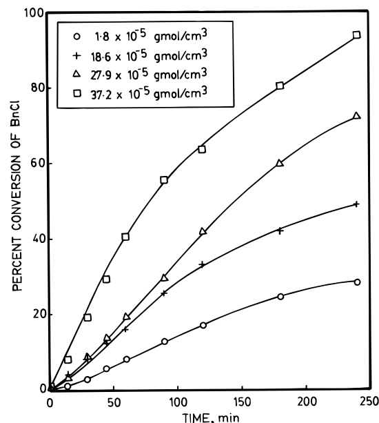
Figure 9. Effect of catalyst concentration on conversion of benzyl chloride. Speed = 1000 rpm. Temperature = 100 °C. [BnCl] = 1.86 \times 10^{-3} mol/cm 3 . [K 2 Cr 2 O 7 ] = 9.33 \times 10^{-4} mol/cm 3 . Vol org = Vol aq = 50 mL. [Na 2 CO 3 ] = 4.44 \times 10^{-4} mol/cm 3 . [TBAB] org = 9.32 \times 10^{-5} mol/cm 3 .
