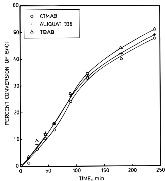
Figure 17. Effect of type of catalyst. Speed = 1000 rpm. Temperature = 100 °C. [BnCl] = 1.86 \times 10^{-3} mol/cm 3 . [K_2Cr_2O_7] = 9.33 \times 10^{-4} mol/cm 3 . Vol_{org} = Vol_{aq} = 50 mL. [Na_2CO_3] = 4.44 \times 10^{-4} mol/cm 3 . [TBAB]_{org} = 9.32 \times 10^{-5} mol/cm 3 .
