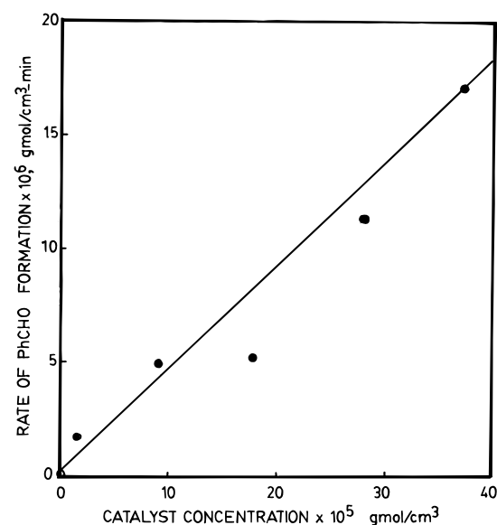
Figure 10. Plot of initial rate of reaction of benzyl chloride against catalyst concentration. Speed = 1000 rpm. Temperature = 100 °C. [BnCl] = 1.86 \times 10^{-3} mol/cm 3 . [K 2 Cr 2 O 7 ] = 9.33 \times 10^{-4} mol/cm 3 . Vol org = Vol aq = 50 mL. [Na 2 CO 3 ] = 4.44 \times 10^{-4} mol/cm 3 . [TBAB] org = 9.32 \times 10^{-5} mol/cm 3 .
