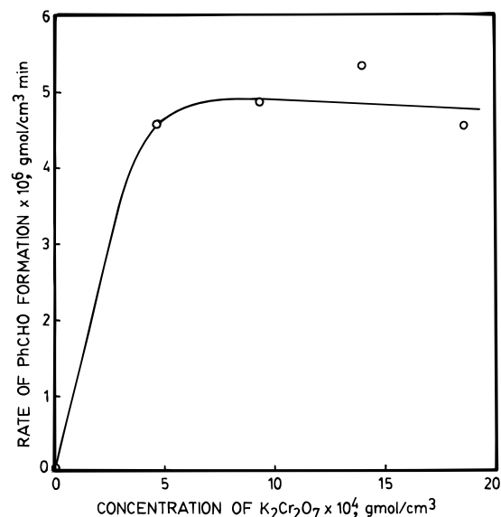
Figure 14. Effect of concentration of nucleophile on the rate of formation of benzaldehyde. Speed = 1000 rpm. Temperature = 100 °C. [BnCl] = 1.86 \times 10^{-3} mol/cm 3 . Vol_{org} = Vol_{aq} = 50 mL. [Na_2CO_3] = 4.44 \times 10^{-4} mol/cm 3 . [TBAB]_{org} = 9.32 \times 10^{-5} mol/cm 3 .
