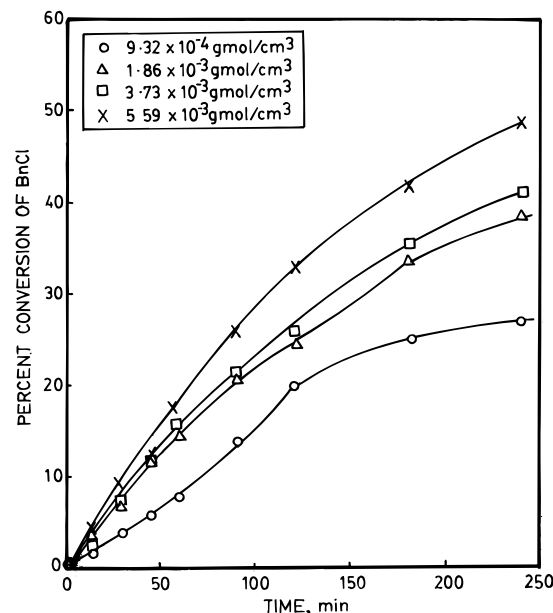
Figure 11. Effect of concentration of benzyl chloride on conversion. Speed = 1000 rpm, Temperature = 100 °C. [K 2 Cr 2 O 7 ] = 9.33 \times 10^{-4} mol/cm 3 . Vol org = Vol aq = 50 mL. [Na 2 CO 3 ] = 4.44 \times 10^{-4} mol/cm 3 . [TBAB] org = 9.32 \times 10^{-5} mol/cm 3 .
