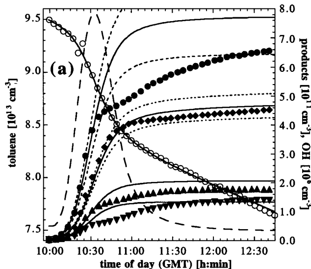
Figure 6. Concentration–time profiles of a toluene/NO photooxidation experiment (3850 ppb toluene, 120 ppb NO). Legend same as for Figure 3.
