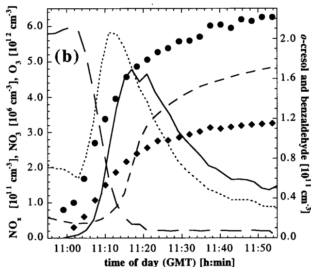
Figure 5. Concentration–time profiles of a toluene/NO photooxidation experiment (690 ppb toluene, 24 ppb NO). Legend same as for Figure 3.
