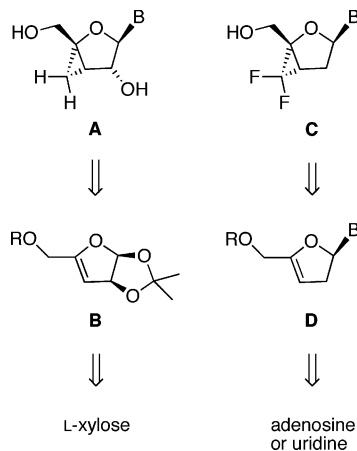
FIGURE 1. 2-Oxabicyclo[3.1.0]hexane analogues.
