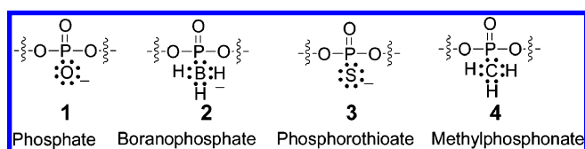
FIGURE 1. Phosphate and its modified analogues.
