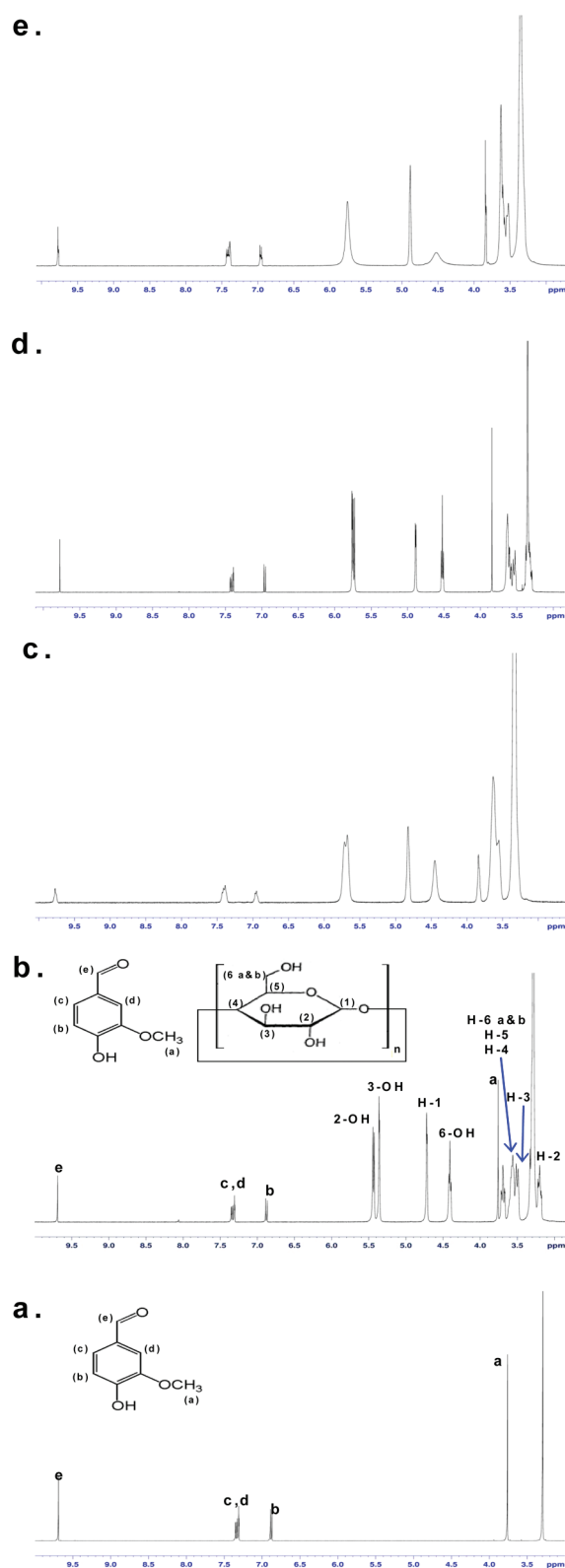
Figure 3. 1 H NMR spectra of (a) vanillin, (b) vanillin/α-CD IC, (c) vanillin/β-CD IC, (d) vanillin/γ-CD IC, and (e) vanillin/γ-CD IC (coprecipitation).
