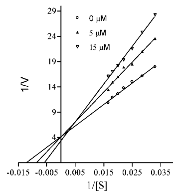
Figure 1. Lineweaver–Burk plot of compound 1 .
