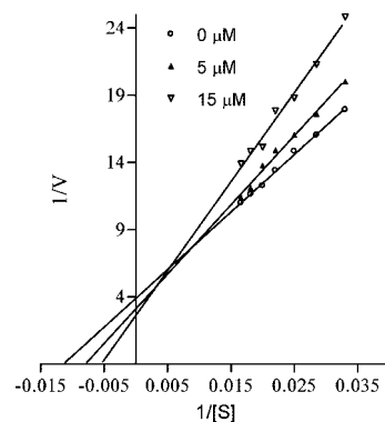
Figure 3. Lineweaver–Burk plot of compound 3 .
