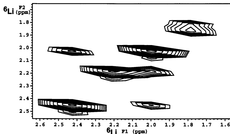
Fig. 5. ^6\text{Li} , ^6\text{Li} -EXSY NMR in \text{DEE-}d_{10} at -60^\circ\text{C} for Li-2 with three equivalents of n -BuLi in excess showing the correlations between signals at \delta 2.03 and 2.46 ppm from the n -BuLi/Li-2 mixed complex.
