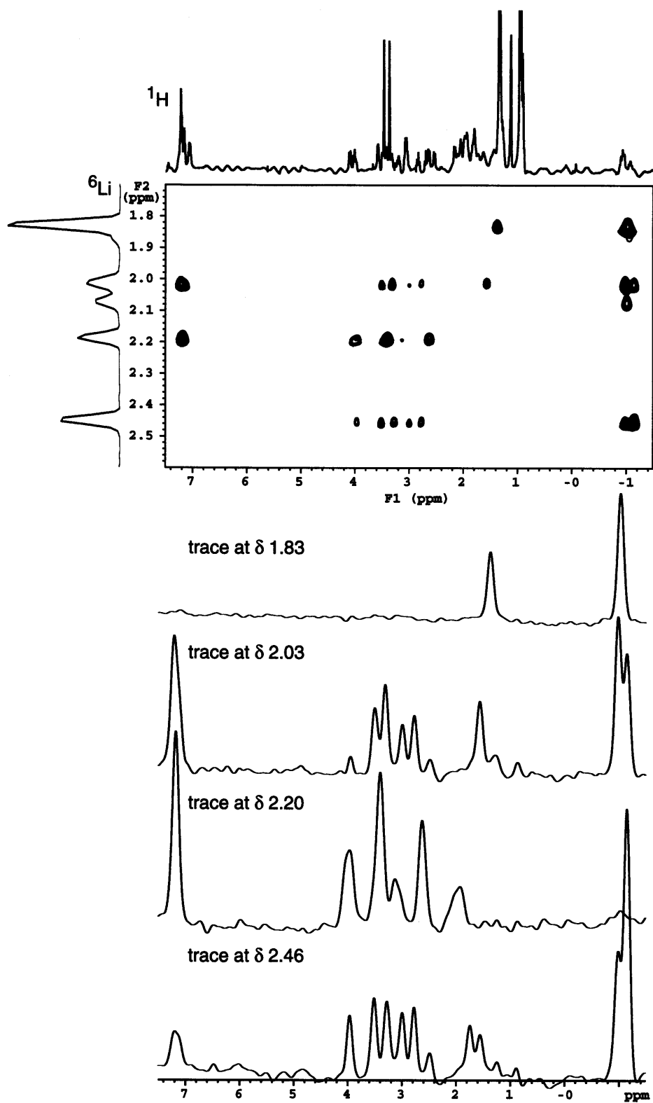
Fig. 4. {}^6\text{Li} , {}^1\text{H} -HOESY NMR in \text{DEE-}d_{10} at -60^\circ\text{C} for Li-2 with three equivalents of n\text{-BuLi} in excess showing the {}^6\text{Li} -NMR traces at \delta 1.83, 2.03, 2.20, and 2.46 ppm.
