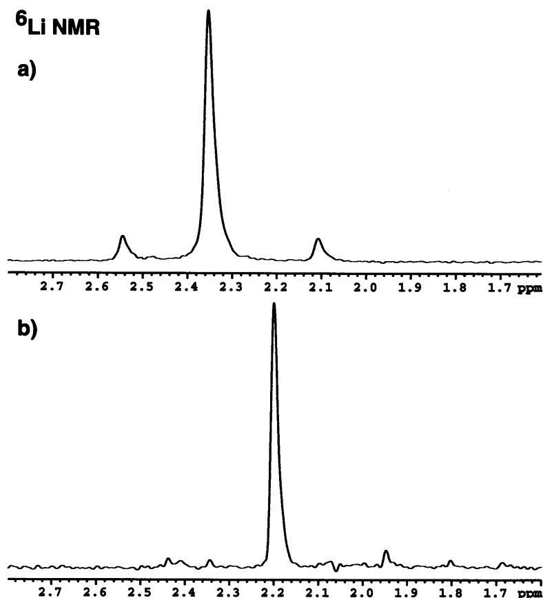
Fig. 1. ^6\text{Li} -NMR in DEE- d_{10} at -60^\circ\text{C} of (a) Li- 1 , (b) Li- 2 .
