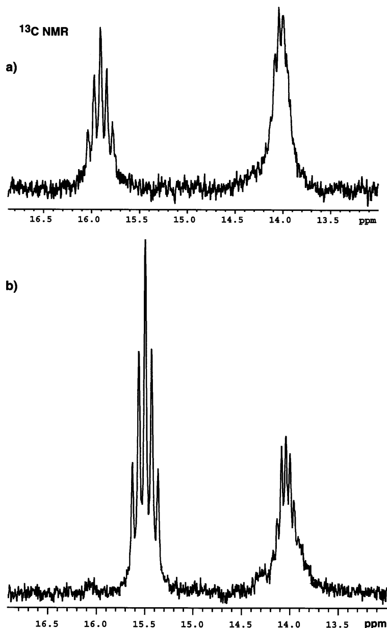
Fig. 6. ^{13}\text{C} -NMR in \text{DEE-}d_{10} at -60^\circ\text{C} of (a) Li-1 with two equivalents of n\text{-BuLi} in excess showing the \alpha -carbon signals from complexed n\text{-BuLi} , at \delta 15.9 ppm (pentet, ^1J_{\text{CLi}} = 8.2 Hz), and free n\text{-BuLi} , at \delta 14.0 ppm (septet, ^1J_{\text{CLi}} = 5.3 Hz), respectively. (b) Li-2 with two equivalents of n\text{-BuLi} in excess showing the \alpha -carbon signals from complexed n\text{-BuLi} , at \delta 15.5 ppm (pentet, ^1J_{\text{CLi}} = 8.3 Hz), and free n\text{-BuLi} , at \delta 14.0 ppm (septet, ^1J_{\text{CLi}} = 5.2 Hz), respectively.
