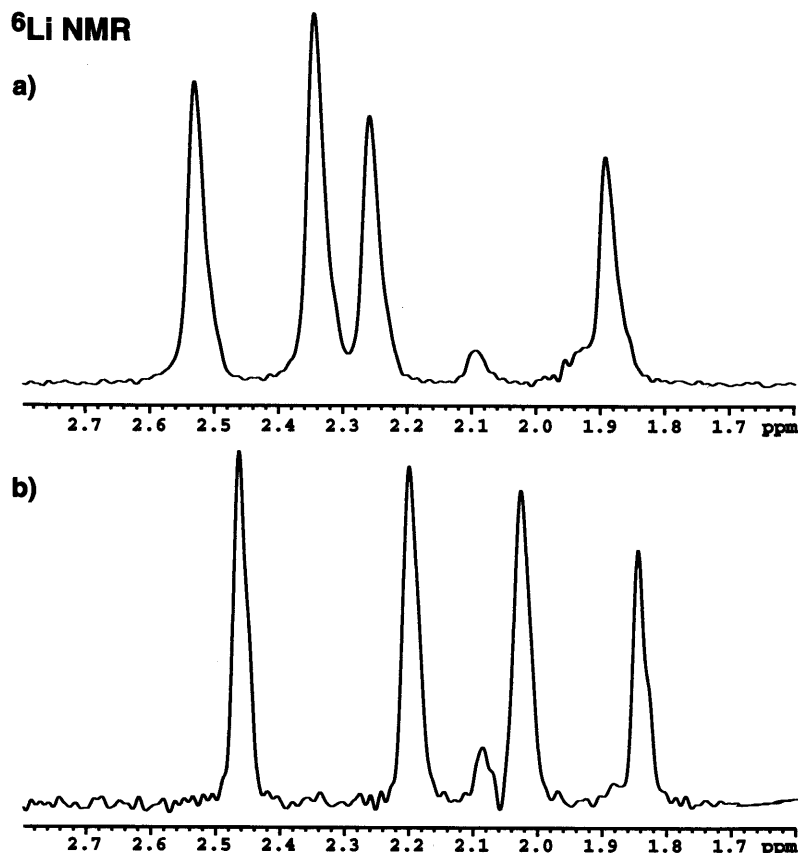
Fig. 2. {}^6\text{Li} -NMR in \text{DEE-}d_{10} at -60^\circ\text{C} of (a) Li-1 with two equivalents of n\text{-BuLi} in excess, (b) Li-2 with three equivalents of n\text{-BuLi} in excess.
