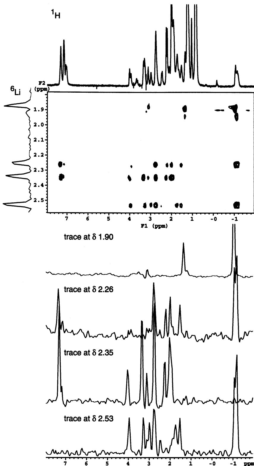
Fig. 3. ^6\text{Li} , ^1\text{H} -HOESY NMR in \text{DEE-}d_{10} at -60^\circ\text{C} for \text{Li-1} with two equivalents of n\text{-BuLi} in excess showing the ^6\text{Li} -NMR traces at \delta 1.90, 2.26, 2.35, and 2.53 ppm.
