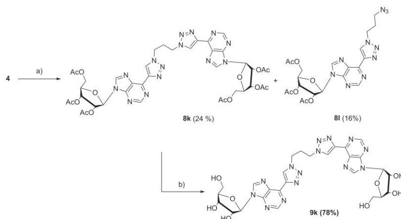
Scheme 5 Reactivity of 4 with 1,3-diazodopropane. (a) CuSO 4 ·5H 2 O, sodium ascorbate, DMF, \mu W, 90 °C, 30 min, 1,3-diazodopropane 7k ; (b) NH 3 , MeOH, rt, 12 h.
