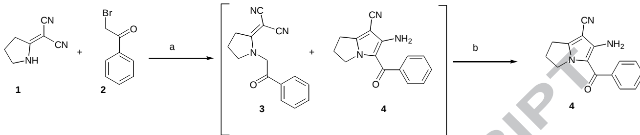
Scheme 1: Synthesis of compound 4 . Reagents and conditions: a) Dry acetone, K_2CO_3 , reflux 20h. b) 1% NaOC_2H_5 , r.t. 24h.
