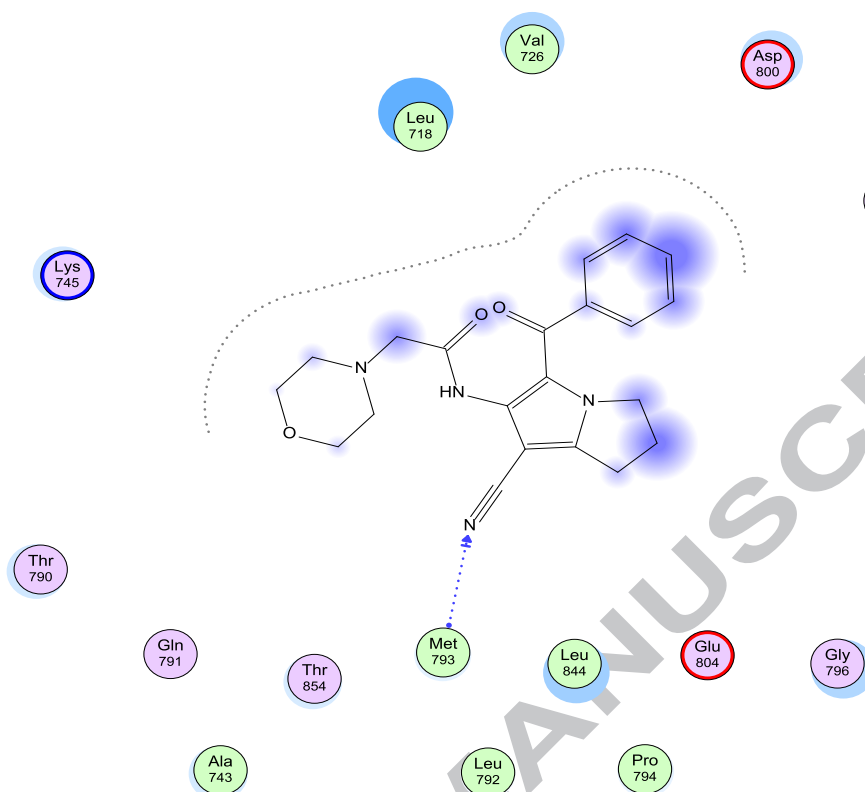
Fig 4. A) 2D interactions of compound 8b with EGFR.
