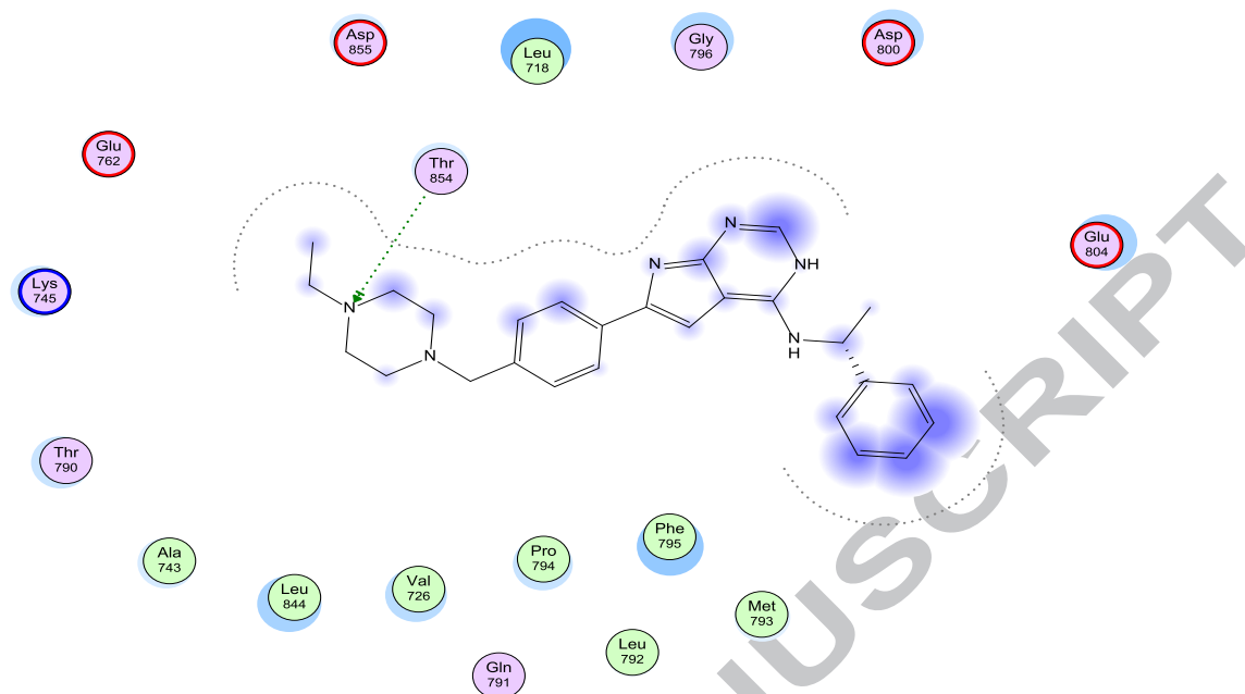
Fig 3. A) 2D interactions of AEE ligand with EGFR.
