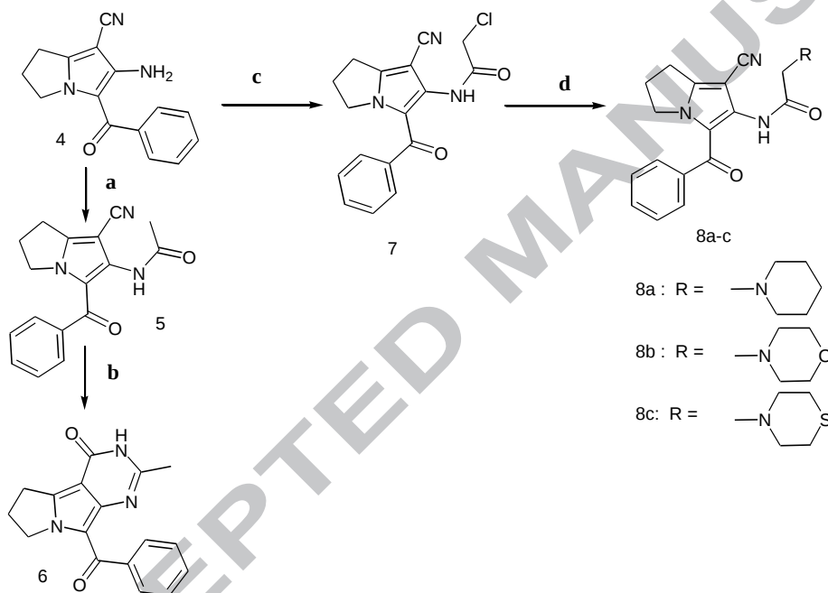
Scheme 2 : Synthesis of compounds 5-8c . Reagents and conditions: a) Acetyl chloride, dioxan, r.t. 24h. b) 1% NaOC_2H_5 , r.t. 24h. c) Chloro acetyl chloride, dioxan, r.t. 12h. d) Secondary amine, abs. ethanol, reflux 24h.
