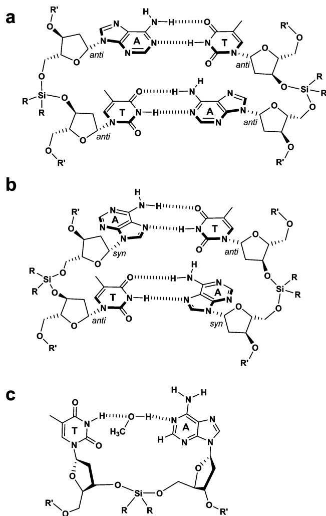
Figure 6. Schematic model for (a) ^1\text{T}_{\text{Si}}\text{A} antiparallel Watson–Crick duplex, (b) ^2\text{T}_{\text{Si}}\text{A} antiparallel Hoogsteen duplex, and (c) putative ^3\text{T}_{\text{Si}}\text{A} -folded dinucleotide structure; R = isopropyl, R' = tert -butyldimethylsilyl.
