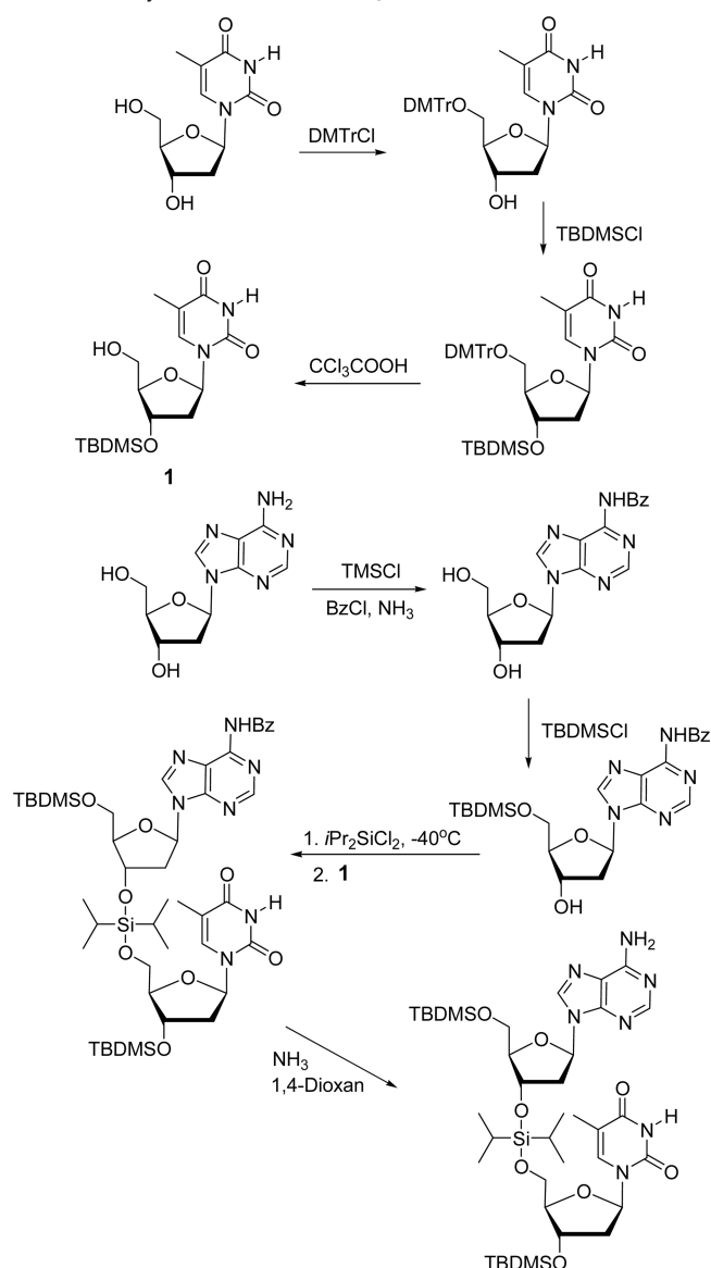
Scheme 1. Synthesis Scheme of A Si T a
