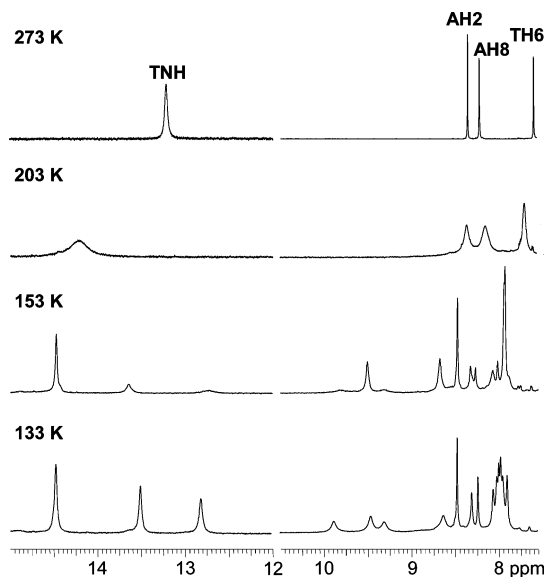
Figure 4. ^1\text{H} NMR spectra of \text{TSiA} in Freon showing base proton spectral regions as a function of temperature.
