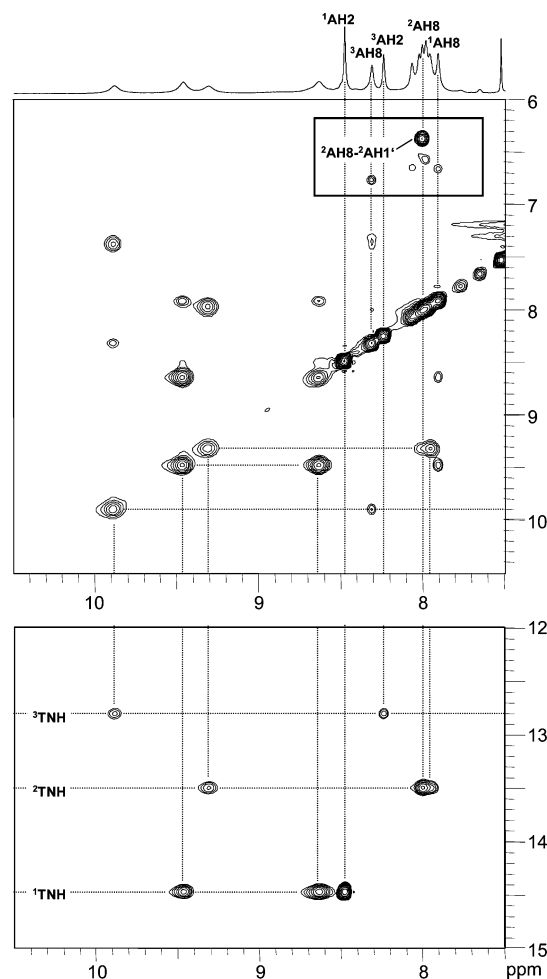
Figure 5. Portion of a 2D NOE spectrum of \text{TSiA} in Freon showing regions with amino/H2/H8-amino/H2/H8/H1' (top) and amino/H2/H8-imino (bottom) crosspeaks. The boxed region encloses base- \text{H1}' contacts. The spectrum was acquired at 133 K with an 80 ms mixing time.
