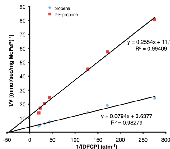
Figure 1. Double-reciprocal Lineweaver–Burk K_m plot for the formation of propene and 2-fluoropropene from DFCP reduction by N_2ase . K_m for both products is the same (0.022 atm, 5.4 mM).
