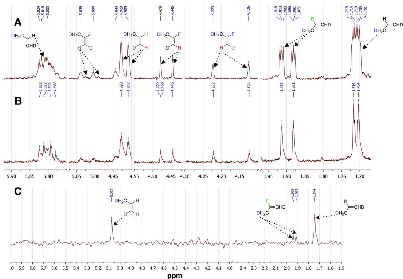
Figure 3. NMR spectra (500 MHz; \text{CDCl}_3/\text{C}_2\text{Cl}_4 = 1:1 ) of products of \text{N}_2\text{ase} -catalyzed reduction of d_2 -DFCP (FeP/MoFeP = 20:1). (A) ^1\text{H} NMR spectrum. (B) ^2\text{H} -decoupled ^1\text{H} NMR spectrum. (C) ^1\text{H} -decoupled ^2\text{H} NMR spectrum.
