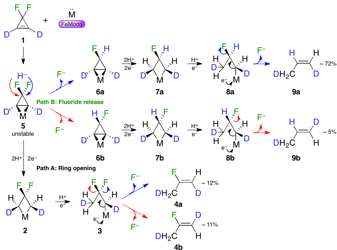
Scheme 2. Proposed Mechanism for Reduction of DFCP Catalyzed by N 2 ase
