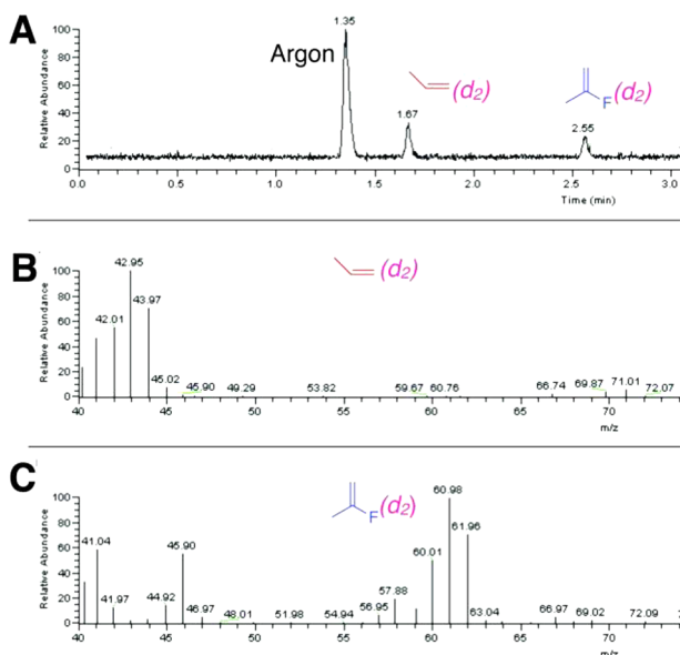
Figure 2. GC-MS spectra of products from d_2 -DFCP reduction by N_2ase (FeP/MoFeP = 20:1). (A) GC chromatogram. (B) MS of P1, identified as d_2 -propene ( [M-H]^+ , m/z = 43 ). (C) MS of P2, identified as d_2 -2-fluoropropene ( [M-H]^+ , m/z = 61 ).
