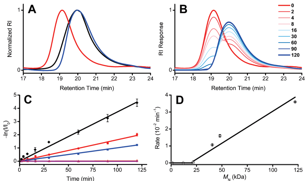
Figure 2. Representative examples of GPC traces and kinetic plots for the mechanochemical scission of [(1)(\text{PyP}_M)_2] . (A) GPC traces of [(1)(\text{PyP}_{66})_2] before and after sonication (red and blue, respectively) overlaid with \text{PyP}_{66} for comparison (black). (B) GPC traces were acquired at timed intervals by analyzing aliquots removed during the sonication of [(1)(\text{PyP}_{66})_2] ( t = 0 , topmost red; the gradual decrease in the peak intensity measured at retention time = 19.13 min ( t = 2 –8 min, fading red) was accompanied by the appearance of a new peak measured at retention time = 19.89 min that was complete after 2 h ( t = 16 –120 min, darkening blue). All aliquots analyzed consisted of an initial polymer concentration of 4 mg mL -1 . (C) First-order rate plot for the sonication of [(1)(\text{PyP}_M)_2] , where M = 66 (black), 25 (red), 21 (blue), 11 (orange), and 7 (purple). I_0 and I correspond to the RI signal prior to sonication and at each time-point t thereafter, respectively. The RI intensity for each polymer was taken at the peak retention times (see Table S2, Supporting Information). (D) Plot of rate coefficients determined in C as a function of M_n . All data points and error bars were calculated from the average and standard deviation, respectively, of three separate experiments.
