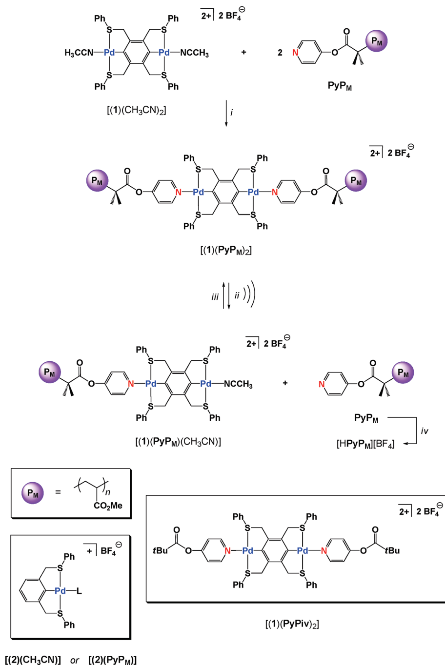
Figure 1. Synthesis and chain scission of mechanoresponsive Pd-based polymers. Conditions: (i) DMF, room temperature, 16 h; (ii) sonication for 2 h at 4 °C of [(1)(\text{PyP}_M)_2] (10 mg) in \text{CH}_3\text{CN} (10 mL), and (iii) recoordination of \text{PyP}_M or (iv) trapping as [\text{HPyP}_M][\text{BF}_4] with 20 equiv of \text{HBF}_4 .
