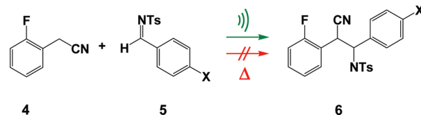
Scheme 1. Palladium-Catalyzed Carbon–Carbon Bond Formation
