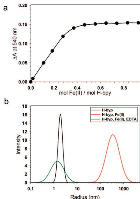
Figure 2. (a) UV-vis titration of H-byp (54 \mu M) with Fe(II); (b) dynamic light scattering of H-byp (1 mM), in 10 mM HEPES pH 7.0 (black), with Fe(II) (500 \mu M) (red), and with Fe(II) (500 \mu M) and EDTA (100 mM) (green).
