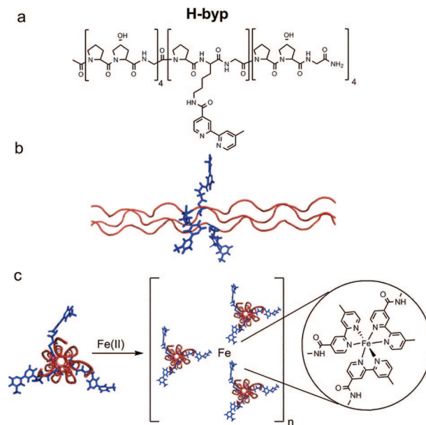
Figure 1. Collagen-mimetic peptide, triple helix, and metal-triggered assembly: (a) amino acid sequence of H-byp ; (b) side view of H-byp after triple helix formation (peptide, red; bipyridine modification, blue); (c) top view of a single triple helix followed by metal-triggered assembly.
