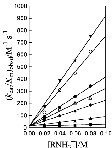
Figure 3. Dependence of (k_{\text{cat}}/K_{\text{m}})_{\text{obsd}} for the K12G mutant TIM-catalyzed isomerization of GAP on the concentration of \text{RNH}_3^+ at pH 7.5, 25 °C, and I = 0.10 (NaCl). Key: (■) \text{NH}_4^+ ; (▲) \text{CH}_3\text{NH}_3^+ ; (◆) \text{CH}_3\text{CH}_2\text{NH}_3^+ ; (△) \text{FCH}_2\text{CH}_2\text{NH}_3^+ ; (●) \text{CH}_3\text{CH}_2\text{CH}_2\text{NH}_3^+ ; (○) \text{MeOCH}_2\text{CH}_2\text{NH}_3^+ ; (▼) \text{CH}_3\text{CH}_2\text{CH}_2\text{CH}_2\text{NH}_3^+ . The slopes of these linear correlation give the third-order rate constants (k_{\text{cat}}/K_{\text{m}})_{\text{am}}/K_{\text{d}} for activation of K12G TIM by \text{RNH}_3^+ (Table 1).
