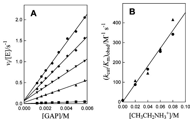
Figure 2. (A) Dependence of the initial velocity, normalized by the concentration of enzyme, of K12G yeast TIM-catalyzed isomerization on the concentration of GAP at various concentrations of added \text{CH}_3\text{CH}_2\text{NH}_3^+ at pH 7.5, 25 °C, and I = 0.10 (NaCl). The slopes of these linear correlations give the apparent second-order rate constant (k_{\text{cat}}/K_{\text{m}})_{\text{obsd}} at the particular concentration of \text{CH}_3\text{CH}_2\text{NH}_3^+ . Key: (■) [\text{EtNH}_3^+] = 0.0 M; (▲) [\text{EtNH}_3^+] = 0.020 M; (▼) [\text{EtNH}_3^+] = 0.040 M; (◆) [\text{EtNH}_3^+] = 0.060 M; (●) [\text{EtNH}_3^+] = 0.080 M. (B) Dependence of the apparent second-order rate constant (k_{\text{cat}}/K_{\text{m}})_{\text{obsd}} for isomerization of GAP catalyzed by K12G yeast TIM on the concentration of added \text{CH}_3\text{CH}_2\text{NH}_3^+ . Key: (●) at pH 7.5; (▲) at pH 7.0.
