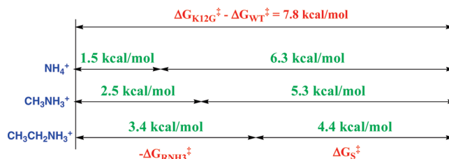
Figure 5. A comparison of the binding energy of primary ammonium cations to the transition state for K12G mutant TIM-catalyzed isomerization of GAP, -\Delta G_{RNH_3}^{\ddagger} , and the apparent transition state stabilization obtained from connecting these activators to the mutant enzyme, \Delta G_S^{\ddagger} . The sum of these terms is equal to the overall stabilization of the transition state for the wildtype TIM-catalyzed isomerization of GAP by interaction with the cationic side chain of Lys-12, \Delta G_{K12G}^{\ddagger} - \Delta G_{WT}^{\ddagger} = 7.8 kcal/mol (eq 6).
