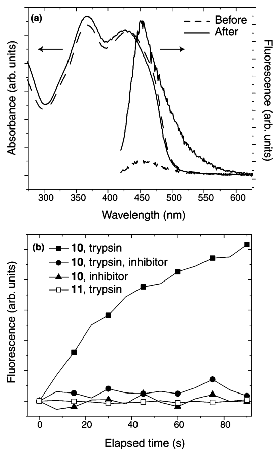
Figure 2. (a) Absorbance (left) and fluorescence (right) spectra of substrate 10 (1.1 \mu\text{M} in repeat units) before and after treatment with trypsin (3 \mu\text{g/mL} ). (b) Generation of fluorescence as a function of time on treatment of 10 and control substrate 11 with trypsin in the absence and presence of an inhibitor (benzamidine hydrochloride).
