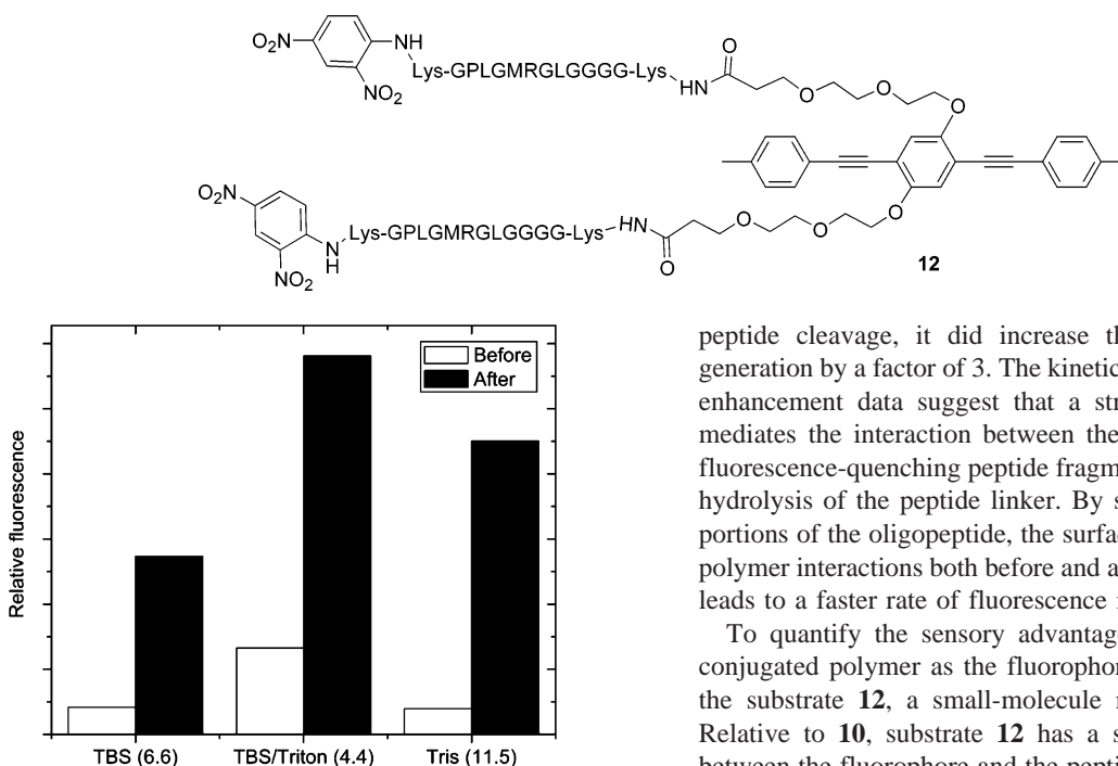
Figure 3. Overall fluorescence enhancement in substrate 10 (0.25 peptide/repeat unit) before and after hydrolysis by trypsin. Numbers in parentheses indicate the overall fluorescence enhancement. TBS: 50 mM Tris, pH 7.5, 150 mM NaCl, and 5 mM CaCl 2 . TBS/Triton: as for TBS, with 0.08% Triton X-100. Tris: 50 mM Tris, pH 7.5.
