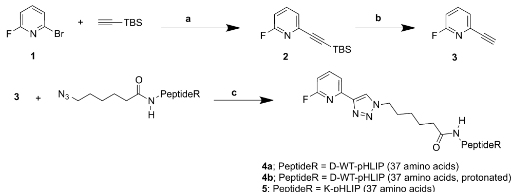
Scheme 1. Synthetic Route Yielding the Non-Radiolabeled Reference Compounds 3 to 5
