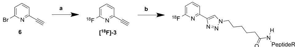
Scheme 2. Radiosynthesis Yielding Radiolabeled Products [ ^{18}\text{F} ]-3 to [ ^{18}\text{F} ]-5
