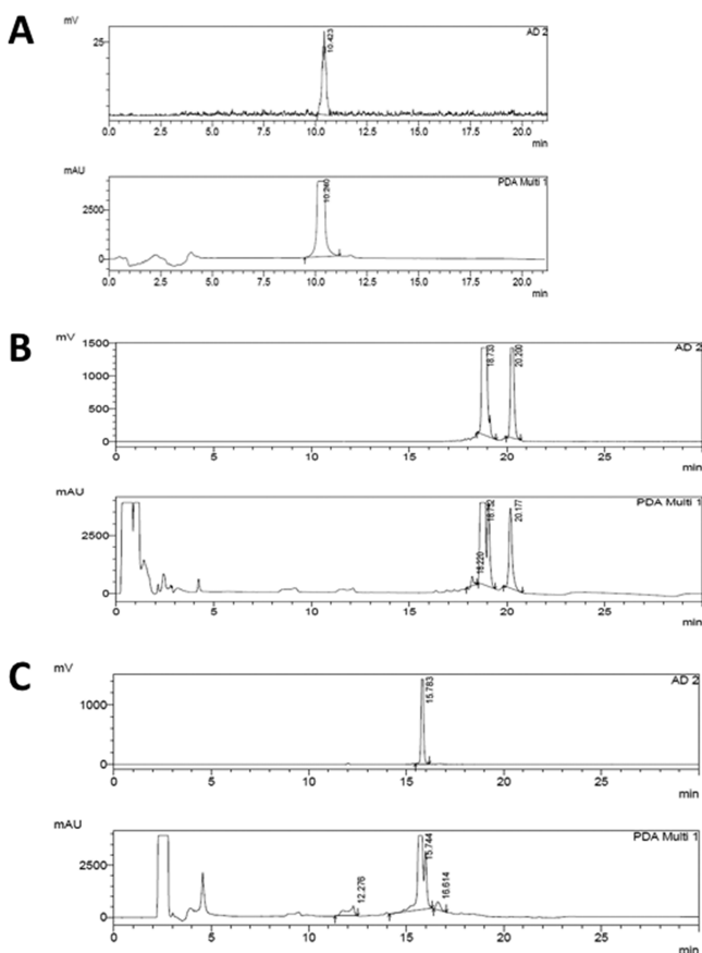
Figure 2. HPLC chromatograms with radio and UV-traces (UV traces were recorded at 254 nm and retention times are given with respect to the radiotrace): (A) coinjection of compound 3 and [ ^{18}\text{F} ]-3 with t_{\text{R}} = 10.4 min on column 1; (B) purification of [ ^{18}\text{F} ]-4a and -4b after 5 min at 70 °C with t_{\text{R}} = 18.7 min and t_{\text{R}} = 20.2 min, respectively; (C) purification of [ ^{18}\text{F} ]-5 after 5 min reaction at 70 °C ( t_{\text{R}} = 15.8 min). HPLC chromatograms were recorded utilizing column 1 applying elution conditions A.
