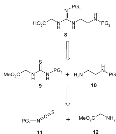
Scheme 5. Retrosynthetic analysis of route A to GuAA.
