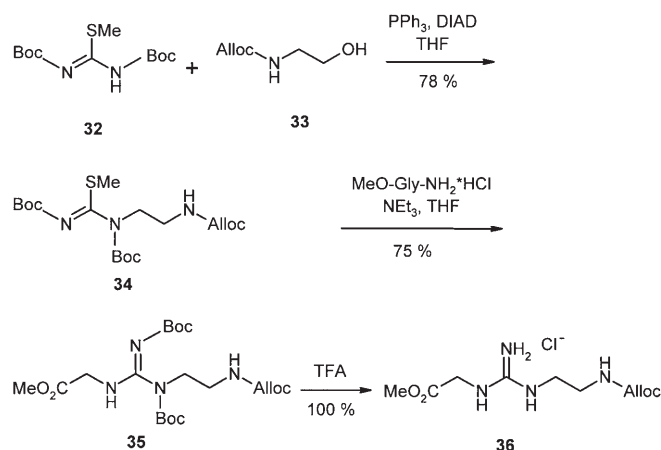
Scheme 11. Synthesis of guanidinium amino ester 36 .
