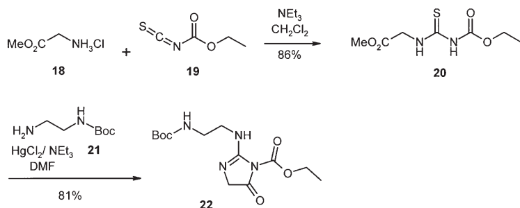
Scheme 7. Synthesis of the cyclic guanidine derivative 22 .
