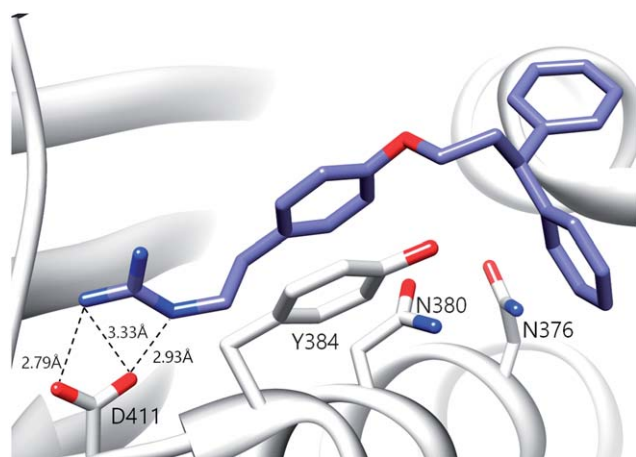
Fig. 4 Predicted binding pose of compound 27 in the active site of HK853. The guanidine moiety of 27 forms a salt-bridge with D411. The ligand is also projected to participate in \pi - \pi stacking interactions with Y384.
