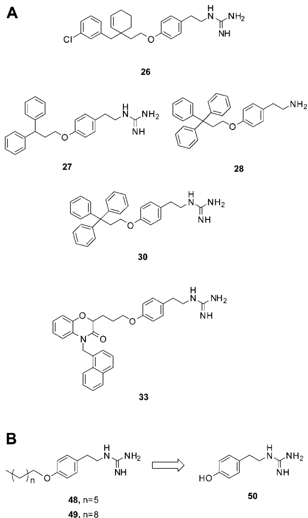
Fig. 3 Compounds bearing guanidine moieties. (A) Subset of compounds predicted to interact with an active site Asp using molecular modeling. (B) Simplified variants of compounds 26, 27, 30 and 33. Further deconstruction of these compounds resulted in the fragment-like compound 50.
