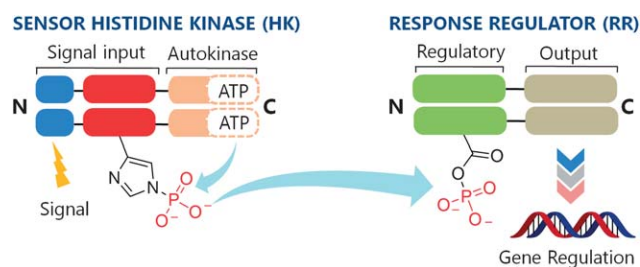
Fig. 1 The two-component system signaling (TCS) cascade. Upon detection of an appropriate signal, autophosphorylation occurs at a conserved His residue of the HK, followed by phosphoryl group transfer to an Asp residue of the RR. A typical function for the RR is gene regulation.
