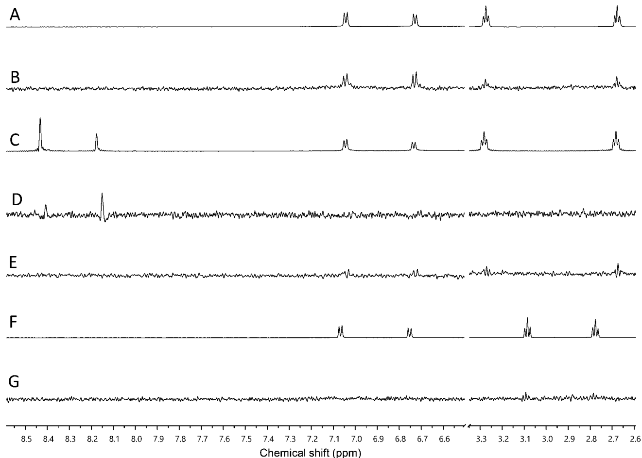
Fig. 7 Assessment of binding using saturation transfer differential (STD) experiments (A) ^1\text{H} spectrum of 50 and HK853, (B) ^1\text{H} STD-NMR spectrum of 50 and HK853, (C) ^1\text{H} NMR spectrum of 50 , ADP and HK853, (D) ^1\text{H} STD-NMR spectrum of 50 , ADP and HK853, (E) ^1\text{H} STD-NMR spectrum of 50 and mutated (D411A) HK853, (F) ^1\text{H} spectrum of tyramine and HK853 and (G) ^1\text{H} STD-NMR spectrum of tyramine and HK853.
