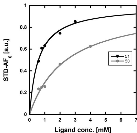
Fig. 8 Determination of the K_d values of compounds 50 and 51 using STD-NMR. Using the initial growth rates approach 53 and mathematical fitting to a Langmuir isotherm, the K_d values of 50 and 51 were found to be 2.41 ( \pm 0.25 ) mM and 0.58 ( \pm 0.06 ) mM, respectively.
