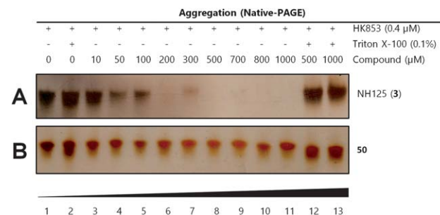
Fig. 6 Gel-based aggregation studies using native-PAGE. (A) NH125 (3) induces aggregation of the protein starting at concentrations as low as 50 μM as evidenced by the disappearance of protein bands and (B) compound 50 does not aggregate HK853 even at concentrations as high as 1 mM.
