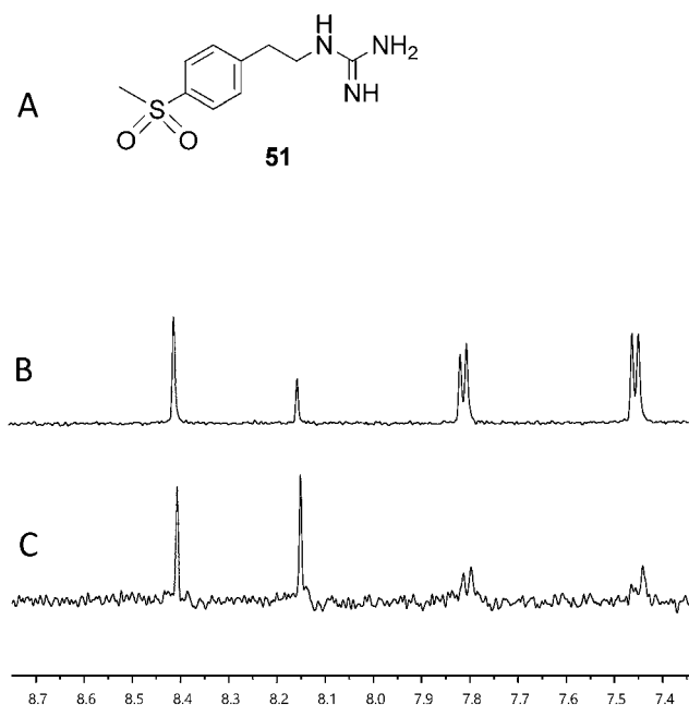
Fig. 9 Assessment of binding using saturation transfer differential (STD) experiments (A) compound 51 , (B) ^1\text{H} spectrum of 51 , ADP and HK853 and (C) ^1\text{H} STD-NMR spectrum of 51 , ADP and HK853.
