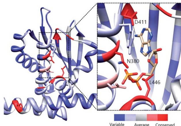
Fig. 5 Evolutionary profile of active site residues in HKs. Derived from the sequence alignment of 150 HK homologs and rendered onto HK853 from Thermotoga maritima . Red colored residues/areas indicate high degrees of evolutionary conservation while blue regions indicate variations in conservation. Inset: Co-crystallized structure of ADP in the CA domain of HK853 (ref. 13) illustrating residues that are involved in binding of the nucleotide. The measured distance between the exocyclic N of ADP and D411 is 2.83 Å.
