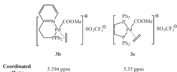
Figure 1. ^1H NMR spectroscopic data [ppm] for the coordinated ethene in 3b and 3c.
