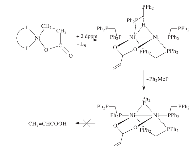
Scheme 4. Reaction of a nickel metallacycle upon treatment with dppm.
