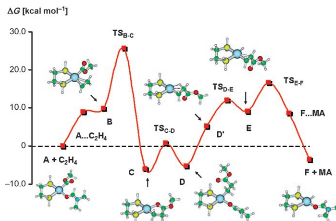
Figure 3. Calculated free energy profile for the formation of methyl acrylate (MA) using the solvated model. For the sake of clarity, the dmf molecule has been omitted for structures B, C, D' and E as it interacts only weakly with the metal centre. The full structures are given in the Supporting Information. Letters A–F are correlated to a–f in Figure 3 but not to a–c in the labeling of the complexes.
