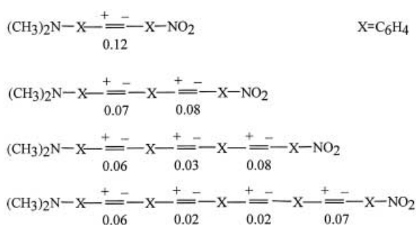
Scheme 5. Polarization of the double bonds in the series (\text{H}_3\text{C})_2\text{N}-\text{OPV}(n)-\text{NO}_2 : Charge differences \Delta q between the olefinic carbon atoms calculated by AM1 ( \Delta q in fractions of the elemental charge, positive and negative signs are related to unsubstituted trans -stilbene).
