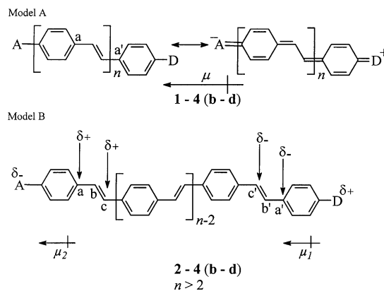
Scheme 4. Models for the push-pull character of the compounds 1–4 ( b–d ): A) VB model indicating the resonance of an electroneutral and a zwitterionic canonical structure; B) MO model with dipolar segments at the chain ends.
