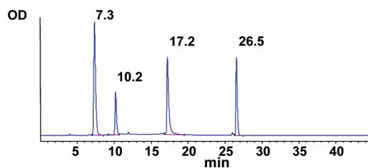
Figure 4. Trace (254 nm) of semipreparative HPLC of the reaction mixture from the formaldehyde-induced coupling of Lys and dG. The peaks at 17.2 and 26.5 min were characterized by NMR. Peaks at 7.3 and 10.2 min are dG and N 2 -hydroxymethyl-dG, respectively.
