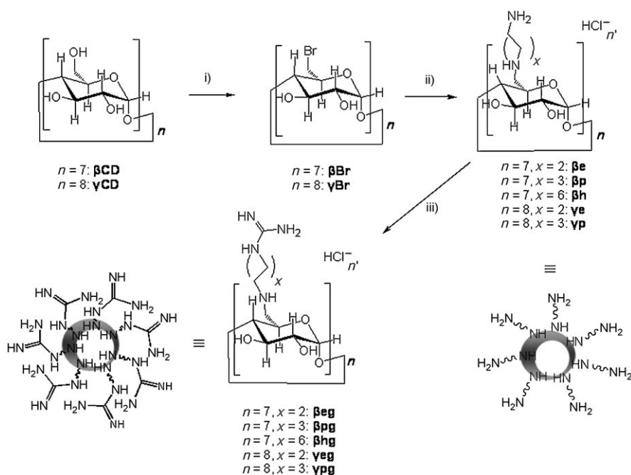
Scheme 2. i) \text{Ph}_3\text{P}/\text{DMF}/\text{Br}_2 , 75–80°C, 18 h; ii) \text{H}_2\text{N}(\text{CH}_2)_x\text{NH}_2 , x=2, 3, 6 , 80°C, 7 atm \text{N}_2 , 3–4 d; iii) 1 H -pyrazole-1-carboxamide·HCl, DMF, DIPEA ( N,N -diisopropylethylamine).
