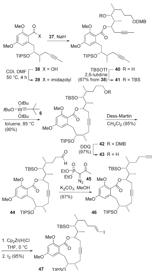
Scheme 10. Synthesis of the macrolactone 47 featuring a 4-iodobutenyl side chain. DDQ = 2,3-dichloro-5,6-dicyano-1,4-benzoquinone.
