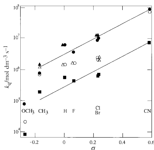
Fig. 9 Semilogarithmic plots of k_{2p} (open symbols) for triplet quenching by propan-2-ol and k_{H_2O} (filled symbols) for quenching by water vs. the Hammett \sigma parameter in acetone (triangles), acetonitrile (circles) and acetic acid (squares) using data from Tables 4 and 5.
