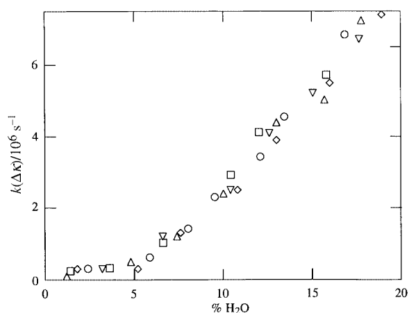
Fig. 7 Rate constant for decay of \Delta K vs. the H 2 O concentration for CN- (○), Br- (◇), Cl- (△), CH 3 - (▽) and OCH 3 -PA (□) in argon-saturated acetonitrile; \lambda_{\text{exc}} = 308 nm.
