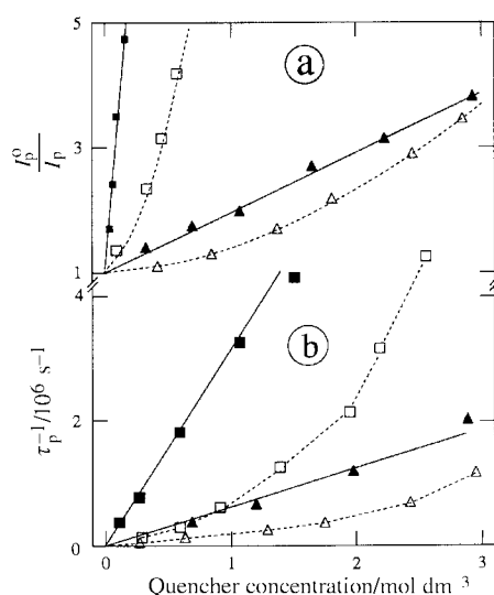
Fig. 3 Plots of (a) I_p^0/I_p and (b) \tau_p^{-1} vs. the quencher concentration for Br-PA (squares) and CH 3 -PA (triangles) in argon-saturated acetonitrile at 25 °C; quencher: propan-2-ol (full symbols) and water (open symbols); \lambda_{\text{exc}} = 340 and 308 nm, for (a) and (b), respectively.
