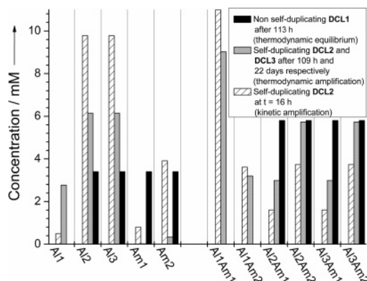
Figure 1. Representation of the products' concentration in various dynamic combinatorial libraries (DCL1–3), determined by ^1\text{H} NMR at 22^\circ\text{C} in \text{CDCl}_3 ( c = 15\text{ mM} for each of the starting materials).
