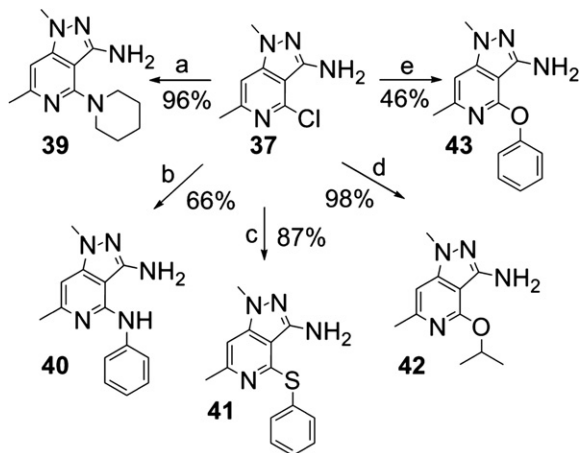
Scheme 12. (a) Piperidine, t BuOH, 160 °C, μW, 30 min; (b) aniline, t BuOH, 160 °C, μW, 30 min; (c) PhSH, K 2 CO 3 , MeCN, reflux, 3 h; (d) NaOPr, i PrOH, reflux, 18 h; (e) PhOH, Cs 2 CO 3 , DMSO, 130 °C, 18 h.
