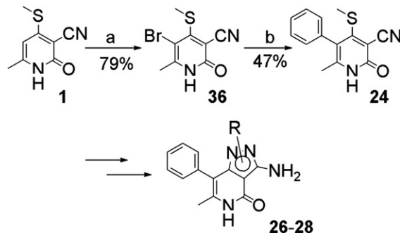
Scheme 10. (a) NBS, MeOH, reflux, 1 h; (b) \text{PhB(OH)}_2 , \text{Pd(PPh}_3)_4 , \text{NaOtBu} , toluene/MeCN (95:5), 150^\circ\text{C} , \mu\text{W} , 1 h.
