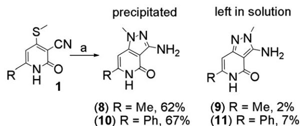
Scheme 3. (a) H(Me)N–NH 2 , Et 3 N, n BuOH, 150 °C, μW, 20 min.
