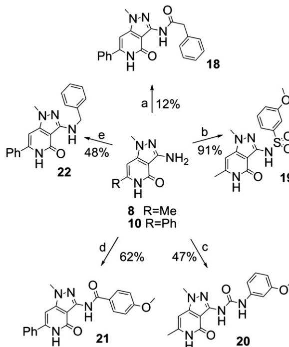
Scheme 5. (a) \text{PhCH}_2\text{COCl} , \text{Et}_3\text{N} , DCM, 0^\circ\text{C} to rt; (b) \text{ArS}(\text{O})_2\text{Cl} , Py, rt, 24 h; (c) \text{ArNCO} , Py, rt; (d) (\text{ArCO})_2\text{O} , Py, 100^\circ\text{C} , 24 h; (e) benzaldehyde, \text{NaBH}_3\text{CN} , AcOH, NaOAc, EtOH/ \text{H}_2\text{O} (1:1), rt.
