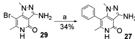
Scheme 8. (a) \text{PhB(OH)}_2 , \text{Pd(PPh}_3)_4 , \text{NaOtBu} , toluene, 150^\circ\text{C} , \mu\text{W} , 1 h.
