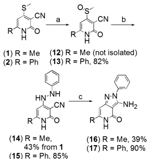
Scheme 4. (a) m -CPBA, EtOH, rt, 24 h; (b) \text{H}_2\text{N}-\text{N}(\text{Ph})\text{H} , i\text{PrOH} , reflux, 2 h; (c) HCl, dioxane, reflux, 3 h.
