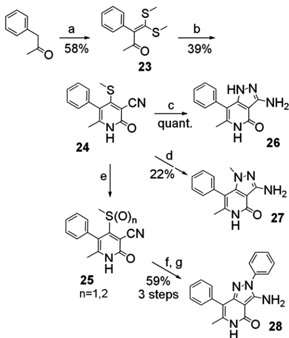
Scheme 6. (a) (i) \text{CS}_2 , \text{NaOtBu} , THF, 0^\circ\text{C} , 5 h; (ii) MeI, MeOH, reflux, 30 min; (b) \text{NCCH}_2\text{CONH}_2 , \text{NaOtPr} , ^i\text{PrOH} , 2 h; (c) \text{H}_2\text{N-NH}_2 , ^i\text{PrOH} , 120^\circ\text{C} , \mu\text{W} , 40 min; (d) \text{H}_2\text{N-N(Me)H} , ^i\text{PrOH} , 150^\circ\text{C} , \mu\text{W} , 1 h; (e) m\text{-CPBA} , EtOH, rt, 18 h; (f) \text{H}_2\text{N-N(Ph)H} , ^i\text{PrOH} , reflux, 2 h; (g) HCl, dioxane, reflux, 30 min.
