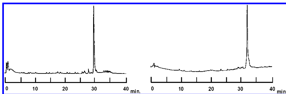
FIGURE 2. Anion exchange HPLC profile of crude cyanoethylated RNAs. (Left) (Uce) 12 . (Right) (GceAceCceUce) 3 .
