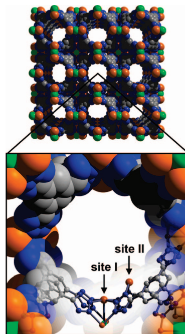
Figure 1. A portion of the crystal structure of 1 showing the two different types of \text{Mn}^{II} sites exposed within its three-dimensional pore system of 10 Å wide channels. 3c Orange, green, gray, and blue spheres represent Mn, Cl, C, and N atoms, respectively; H atoms and bound MeOH molecules are omitted for clarity. Site I is five-coordinate, while site II is only two-coordinate; the separation between them is 3.420(8) Å.
