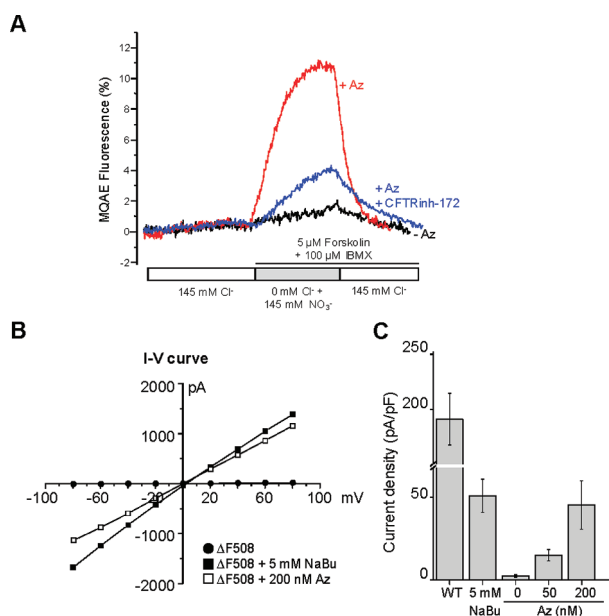
Figure 7. Az restores the \text{Cl}^- channel activity of \Delta\text{F508} -CFTR. (A) Cyclic AMP-dependent chloride channel activities were examined by measuring intracellular chloride concentration changes with MQAE. (B) The current–voltage ( I – V ) relationships. Whole cell current was measured by using a patch-clamp technique in \Delta\text{F508} -CFTR HEK cells that were untreated or treated with 5 mM NaBu or 200 nM Az. (C) The dose-dependent \text{Cl}^- channel activity of \Delta\text{F508} -CFTR. Peak currents were normalized as currents densities (pA/pF).
