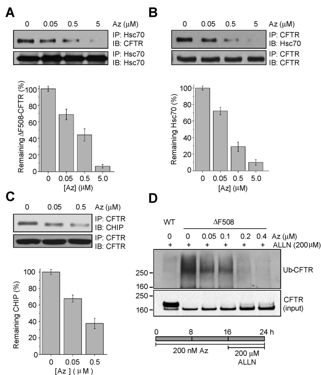
Figure 8. Az inhibits the interaction between \Delta\text{F508} -CFTR and Hsc70 and CHIP to suppress ubiquitination of the mutant protein. Az treatment of \Delta\text{F508} -CFTR HEK cells decreases the amount of (A) mutant CFTR coprecipitated with Hsc70, (B) Hsc70 coprecipitated with CFTR, and (C) CHIP coprecipitated with CFTR. (A–C) Lysates of \Delta\text{F508} -CFTR HEK cells were exposed to various concentrations of Az for 1 h at 25 °C (mean \pm SD). (D) Suppression of ubiquitination of mutant CFTR by Az. CFTR and \Delta\text{F508} -CFTR HEK cells were treated with various concentrations of Az for 24 h at 37 °C. Proteasomal degradation of ubiquitinated CFTRs was blocked by 200 \mu\text{M} ALLN.
