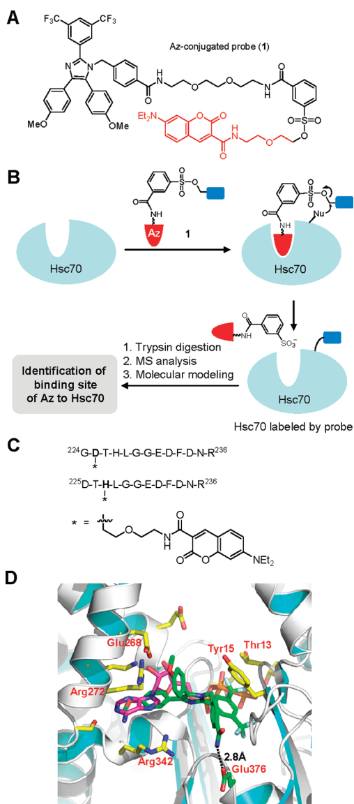
Figure 3. (A) Chemical structure of Az-conjugated probe 1. (B) Schematic illustration of the strategy used to identify the binding site of Hsc70 for Az using 1. Binding of 1 to Hsc70 promotes protein labeling via an S_N2 -type reaction. The binding site of Hsc70 for Az can be identified by mass spectrometry after trypsin digestion (Nu: a nucleophilic amino acid residue). (C) Sequence of the labeled peptides identified by nanoLC-MS/MS analysis. His227 (major) and Asp225 (minor) were labeled by a fragment of 1. (D) Docking model of Az (green)/Hsc70 (PDB code 3FZM) superimposed with ATP (red, adenosine; orange, triphosphate).
