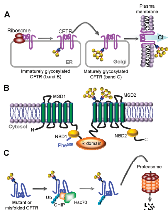
Figure 1. (A) Trafficking of folded wt-CFTR to the plasma membrane. Immaturely glycosylated CFTR (band B) in the ER moves to the Golgi where maturely glycosylated CFTR (band C) is formed. The mature form of CFTR is translocated to the plasma membrane to act as a chloride channel. (B) Representation of CFTR structure inserted into the plasma membrane (MSD, membrane-spanning domain; R domain, regulatory domain; NBD, nucleotide-binding domain; N, amino terminus; C, carboxy terminus). Two N-glycans are also indicated. (C) ER-associated degradation of mutant or misfolded CFTR. Mutant or misfolded CFTR is strongly recognized by Hsc70 followed by CHIP that has the ubiquitin (Ub) ligase activity. The ubiquitinated CFTR is removed by 20S proteasome.
