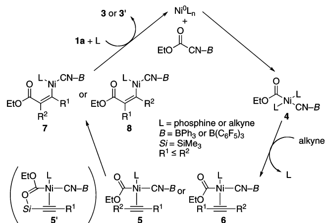
Scheme 2. Transformations of 3'ae a
