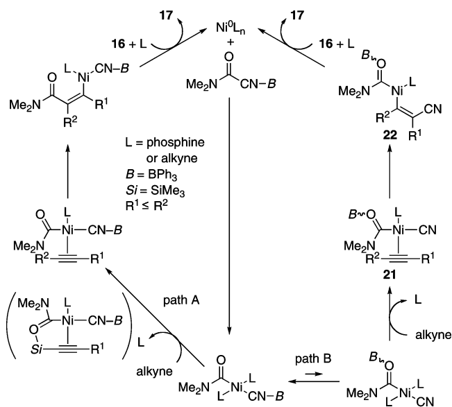
Scheme 5. Plausible Mechanism of Cyanocarbamoylation of Alkynes by Nickel/LA Catalysis
