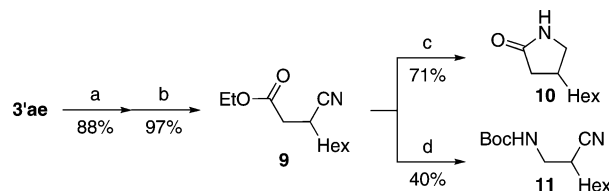
Scheme 2. Transformations of 3'ae a
