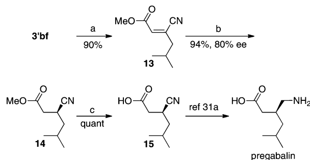
Scheme 3. Formal Synthesis of Pregabalin a
