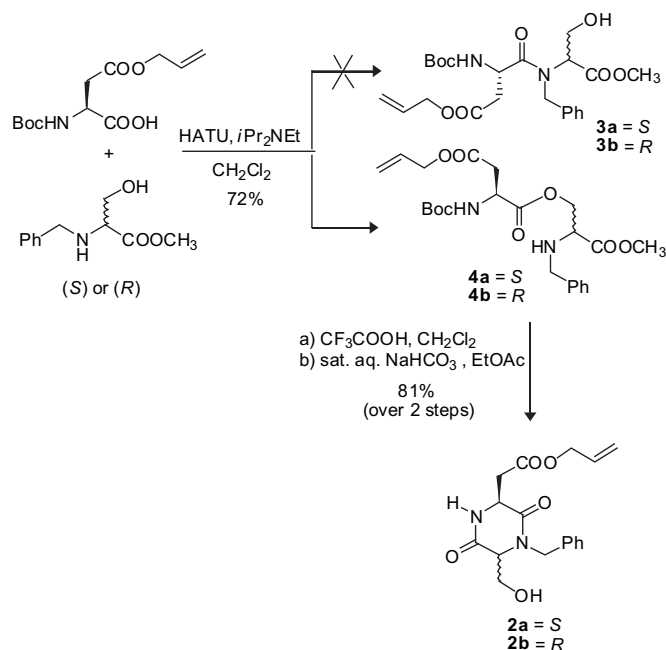
Scheme 2. Coupling of N -( tert -butoxycarbonyl)-(2 S )-aspartic acid \beta -allyl ester with either ( S )- or ( R )- N -benzylserine methyl ester.
