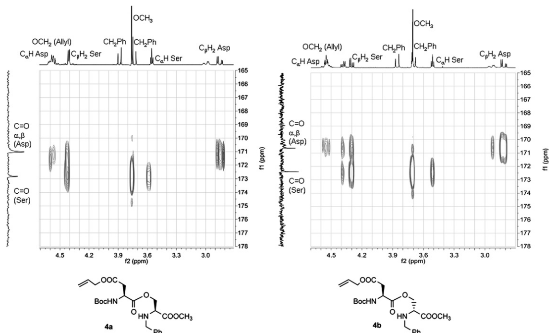
Fig. 1. HMBC spectra of isopeptides 4a ( \text{CDCl}_3 ) and 4b ( \text{CD}_2\text{Cl}_2 ), highlighting the long range coupling (through three bonds) between the \text{O}-\text{CH}_2 protons of Ser and the \alpha -carbonyl carbon of Asp.
