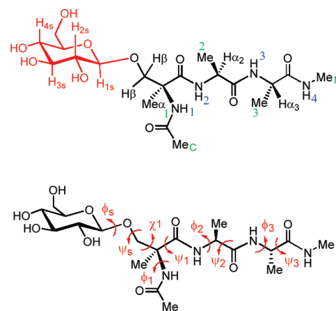
FIGURE 2. Molecular structure of glycopeptide 4 , showing the atom labels and the most relevant torsional angles. The letter “s” makes reference to the sugar moiety. The blue and green numbers refer to the numeration of the NH and methyl groups, respectively. The same atom labels were used for the rest of the molecules.
