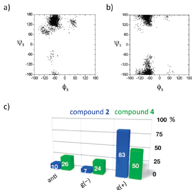
FIGURE 5. (a) \phi_s/\psi_s ( s = sugar) distribution obtained from the MD-tar simulations for compound 2 . (b) \phi_s/\psi_s distribution obtained from the MD-tar simulations for compound 4 . (c) \chi^1 distribution obtained from the MD-tar simulations for compounds 2 and 4 .
