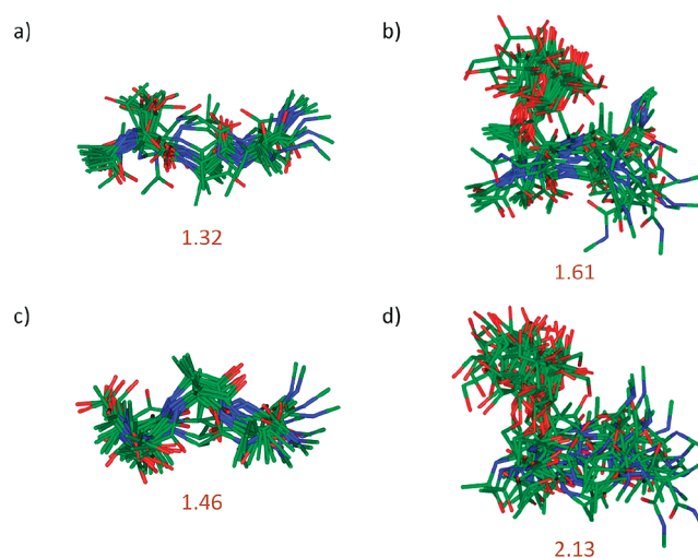
FIGURE 6. Calculated ensembles obtained from the MD-tar simulations for peptide 1 (a), glycopeptide 2 (b), peptide 3 (c), and glycopeptide 4 (d), showing the RMSDs for heavy atoms superimposition.
