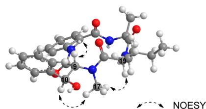
Figure 1. Key NOESY correlations of compound 1 .
